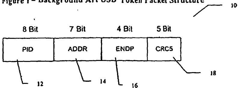
Figure 1 – Background Art USB Token Packet Structure
