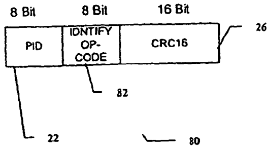
Fig 7 – Flash Identification Request Packet
