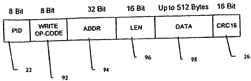
Fig 9 – Write Request Packet
