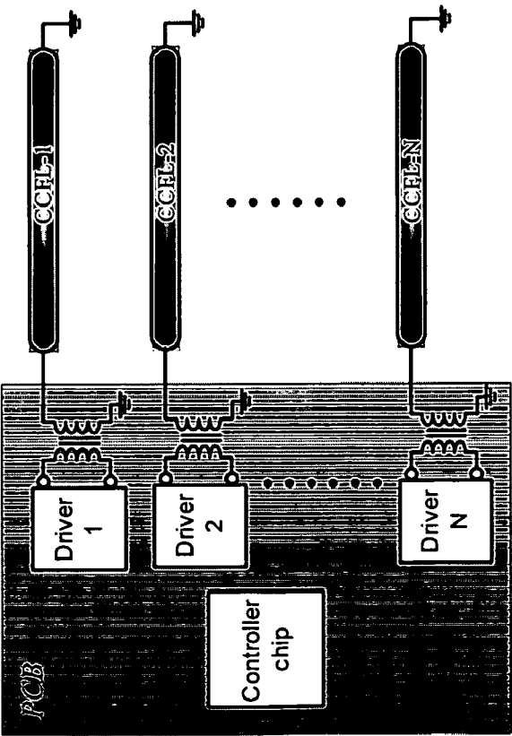
Fig. 7 (Related Art)
