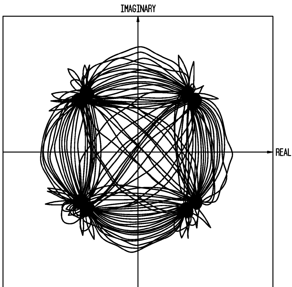
FIG. 30 I/Q MEASURED POLAR VECTOR
