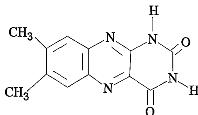
7,8-dimethylalloxazine
