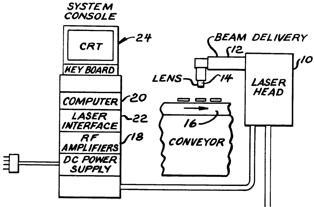
SYSTEM CONFIGURATION FIG. 1
