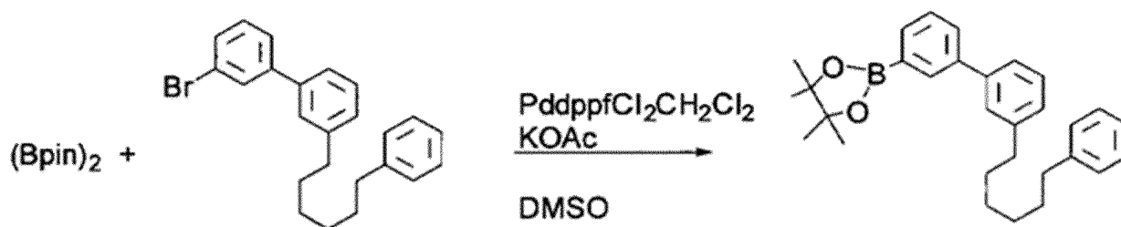
(Intermediate 1)
