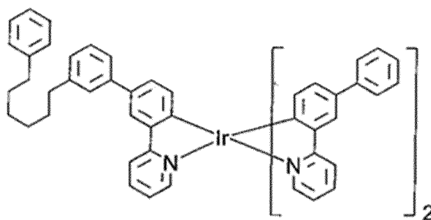
(Compound D-5)
