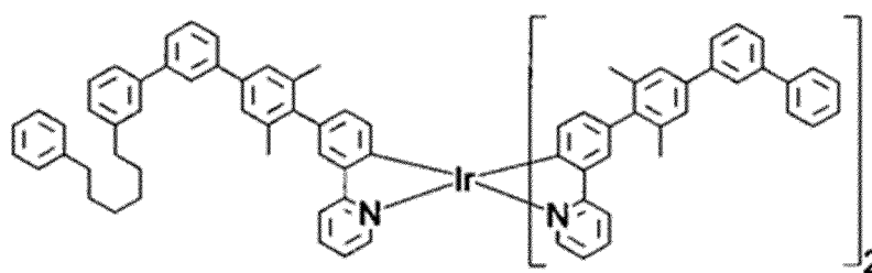
(Compound D-2)
