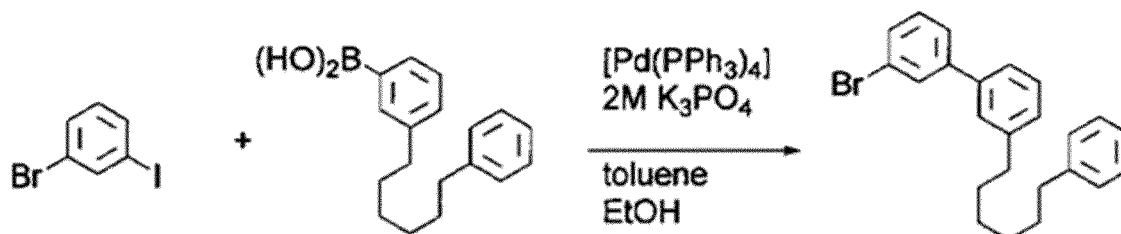
(Intermediate 1)
