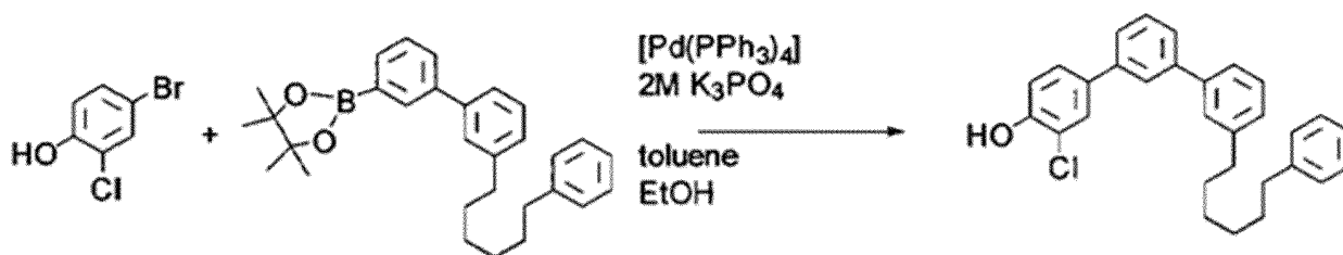
(Intermediate 3)
