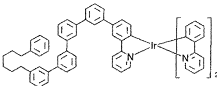
(Compound D-6)
