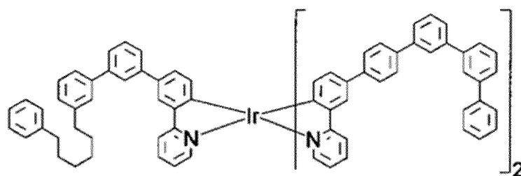
(Compound D-1)
