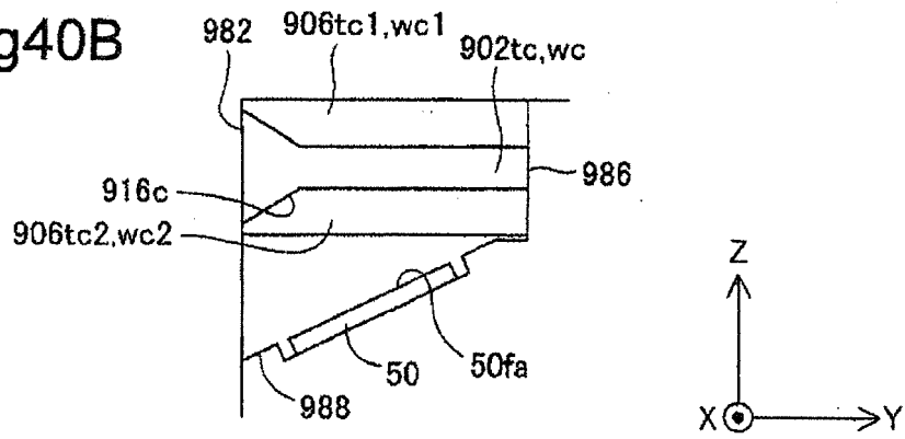
40-40 CROSS-SECTIONAL VIEW
