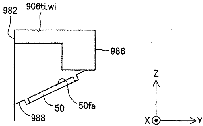
46-46 CROSS-SECTIONAL VIEW
