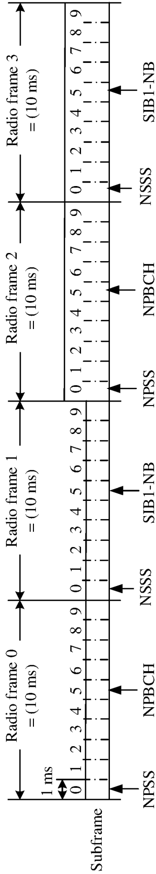
Radio frame using a TDD technology
