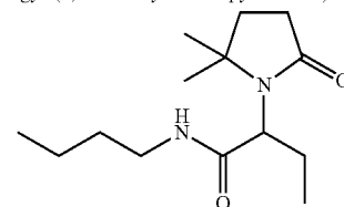
N-n-butyl-2-(5,5-dimethyl-2-oxo-pyrrolidino)-butyramide;
