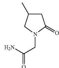
(4-methyl-2-oxo-pyrrolidino)-acetamide;
