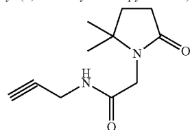
N-propargyl-(5,5-dimethyl-2-oxo-pyrrolidino)-acetamide;
