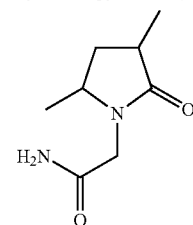
(3,5-dimethyl-2-oxo-pyrrolidino)-acetamide;
