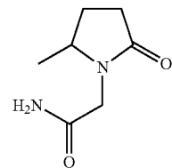
(5-methyl-2-oxo-pyrrolidino)-acetamide;
