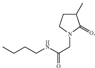
N-n-butyl-(3-methyl-2-oxo-pyrrolidino)-acetamide;
