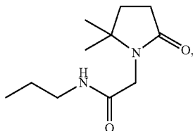
N-n-propyl-(5,5-dimethyl-2-oxo-pyrrolidino)-acetamide;
