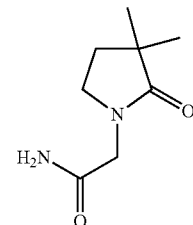
(3,3-dimethyl-2-oxo-pyrrolidino)-acetamide;
