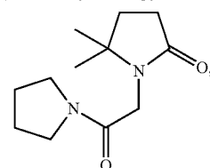
N-[(5,5-dimethyl-2-oxo-pyrrolidino)-acetyl]-pyrrolidine;
