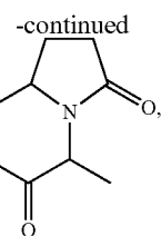
2-(5-methyl-2-oxo-pyrrolidino)-propionamide;
