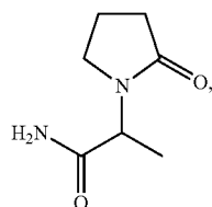
2-(2-oxo-pyrrolidino)-propionamide;
