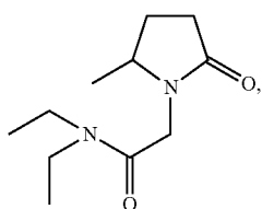
(5-methyl-2-oxo-pyrrolidino)-N,N-diethylacetamide;
