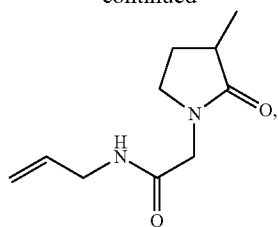
N-allyl-(3-methyl-2-oxo-pyrrolidino)-acetamide;
