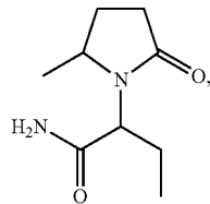
2-(5-methyl-2-oxo-pyrrolidino)-butyramide;
