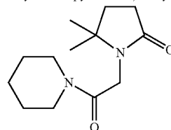
N-[(5,5-dimethyl-2-oxo-pyrrolidino)-acetyl]-piperidine; and
