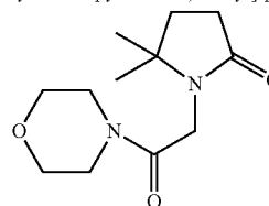
N-[(5,5-dimethyl-2-oxo-pyrrolidino)-acetyl]-morpholine.
