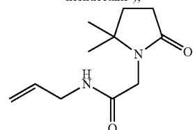
N-allyl-(5,5-dimethyl-2-oxo-pyrrolidino)-acetamide;
