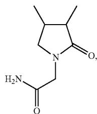
(3,4-dimethyl-2-oxo-pyrrolidino)-acetamide;
