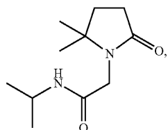
N-isopropyl-(5,5-dimethyl-2-oxo-pyrrolidino)-acetamide;
