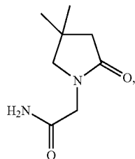
(4,4-dimethyl-2-oxo-pyrrolidino)-acetamide;
