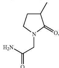
(3-methyl-2-oxo-pyrrolidino)-acetamide;
