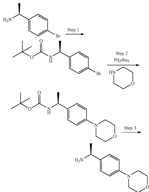
Step 1: Synthesis of [(S)-1-(4-bromo-phenyl)-ethyl]-carbamic Acid Tert-Butyl Ester
