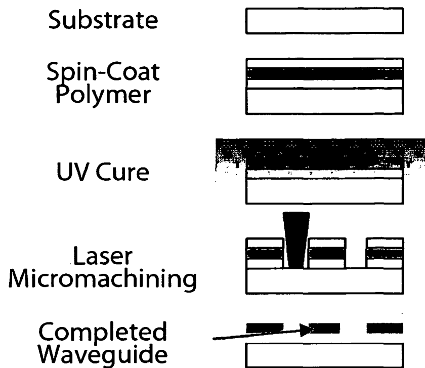
Fabrication of 3-Layer Planar Waveguide
