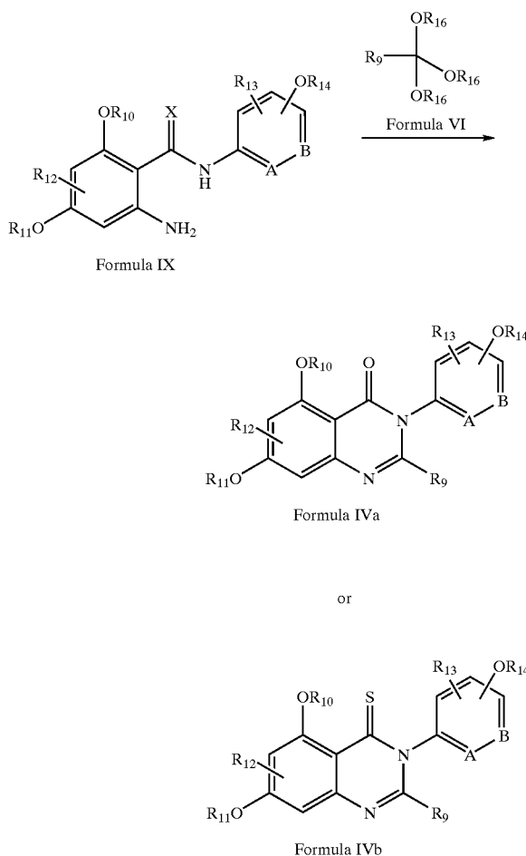
Reaction Scheme 2a
