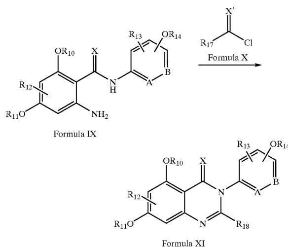
Reaction Scheme 2b
