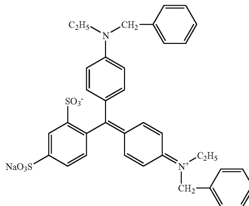
Blue dye 1
