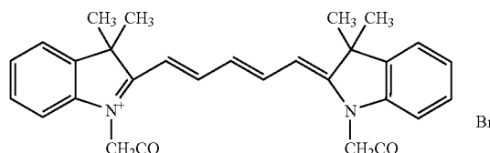
Cyanine compound 1
