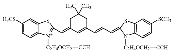
p-Ts-
