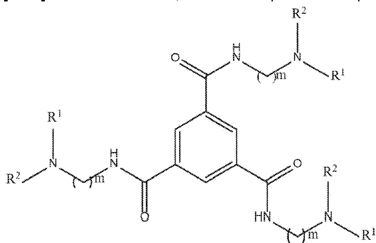
Formula Ia
