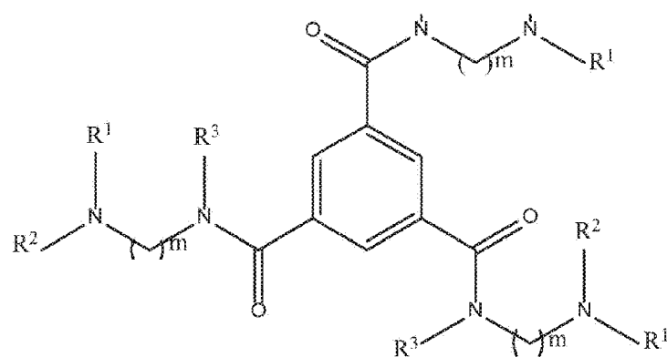
Formula I
