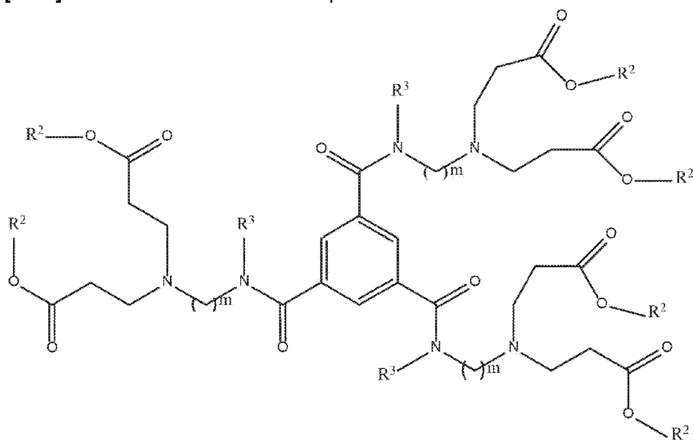
Formula IV
