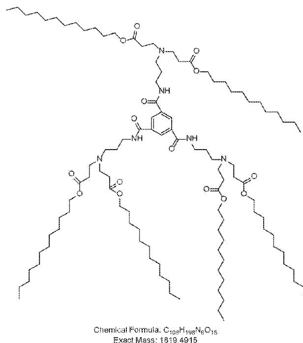
Compound III-1
