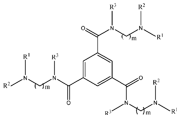
Formlen I
