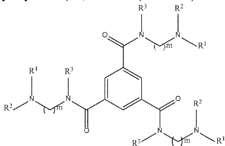
Formula I
