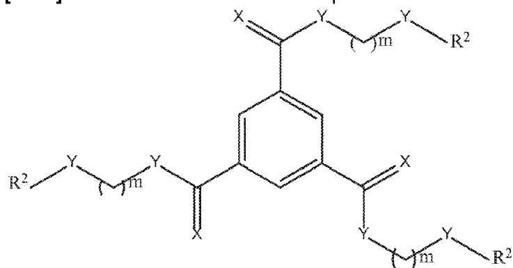
Formula II
