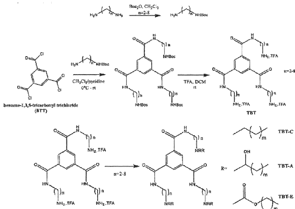
Scheme 4
