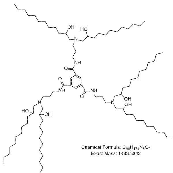
Compound III-1
