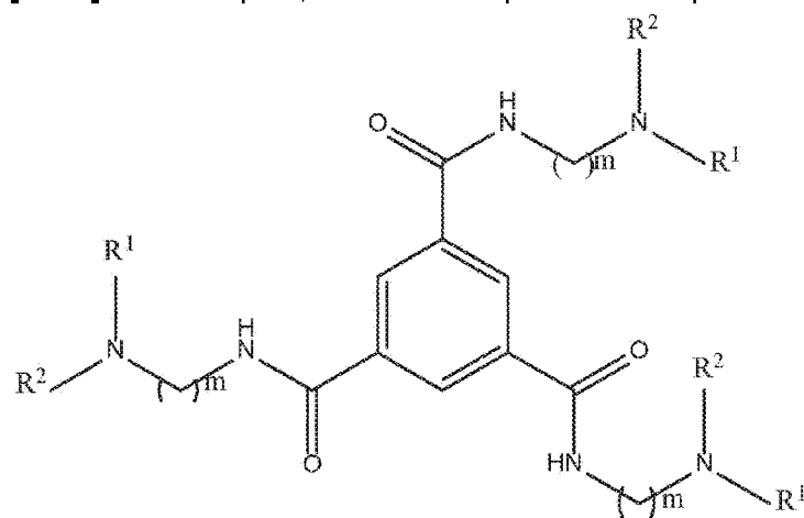
Formula Ia
