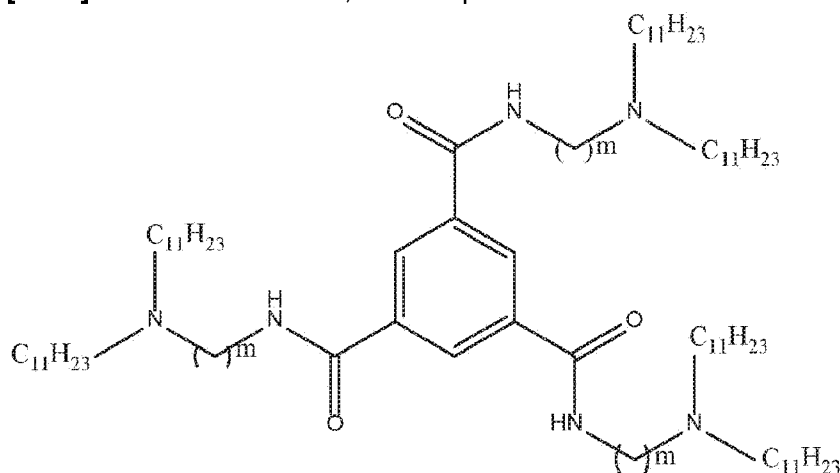
Compound TT3
