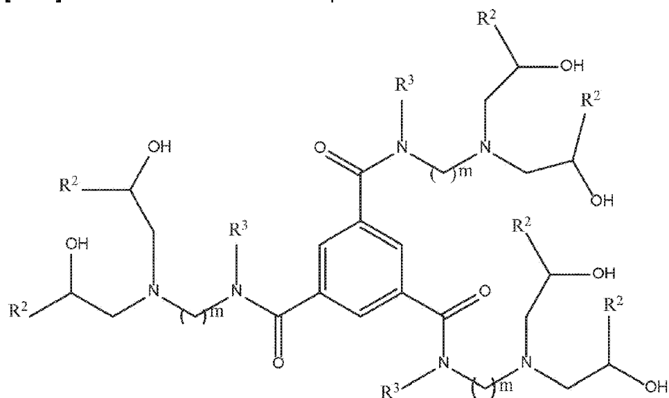
Formula III
