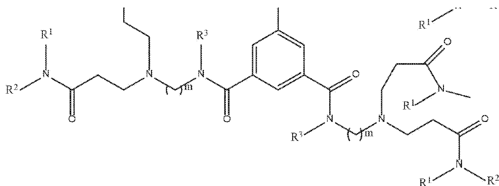
Formula V
