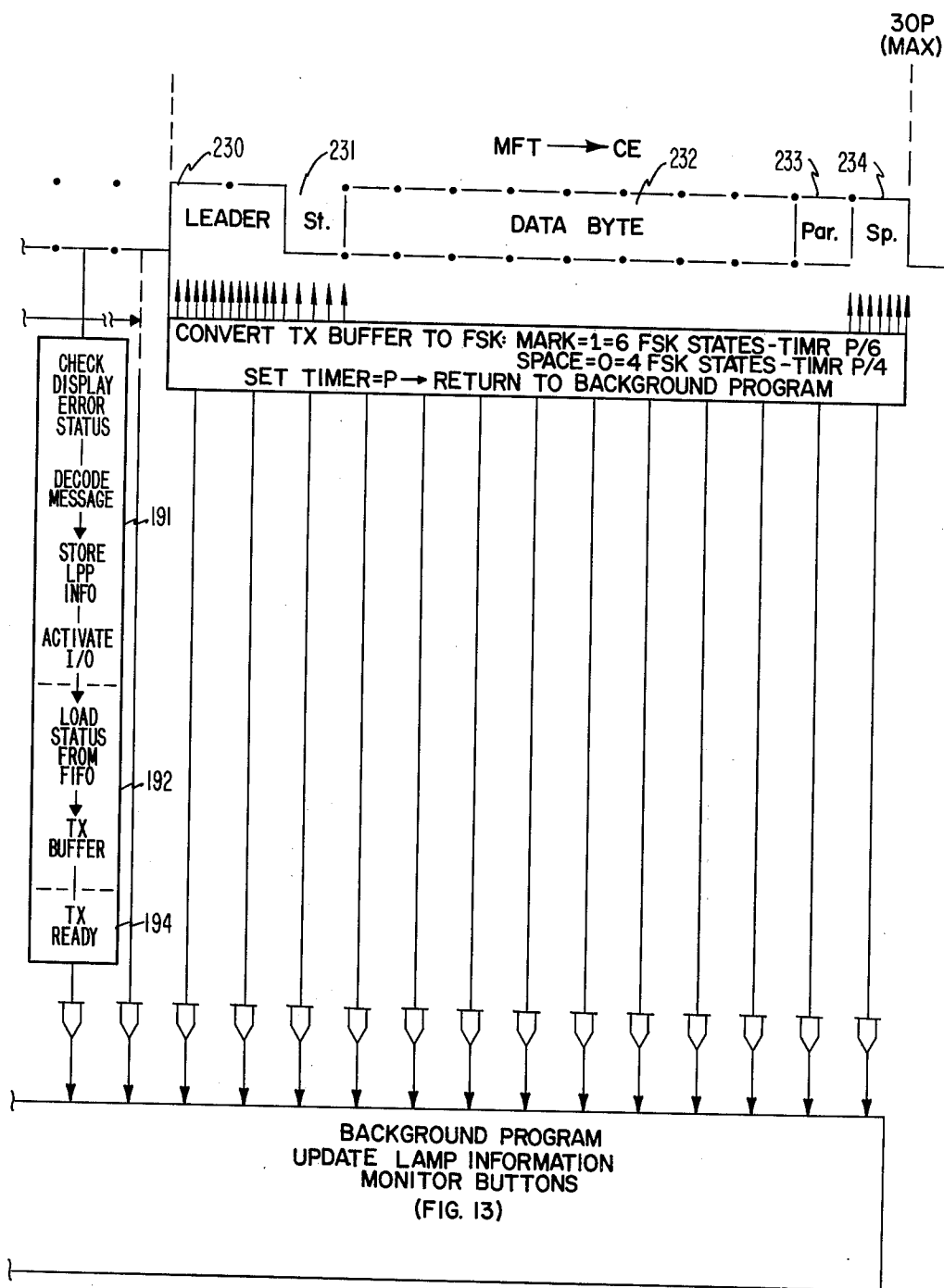
FIG. 12B MULTIFUNCTION TELEPHONE/ COMMON EQUIPMENT (CB) INFORMATION CYCLE
