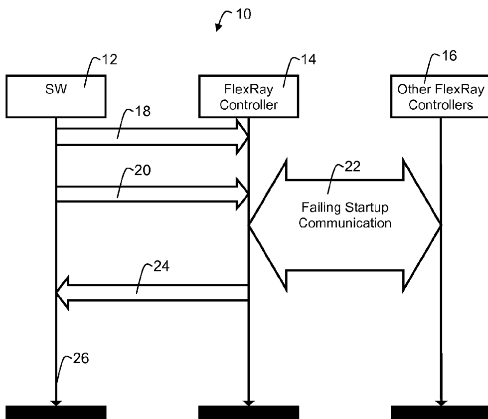
FIG. 1 (PRIOR ART)
