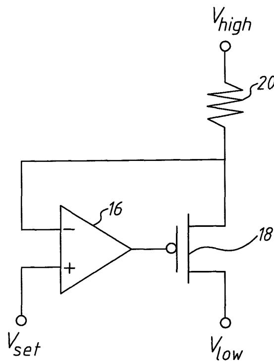
Fig. 2 (prior art)
