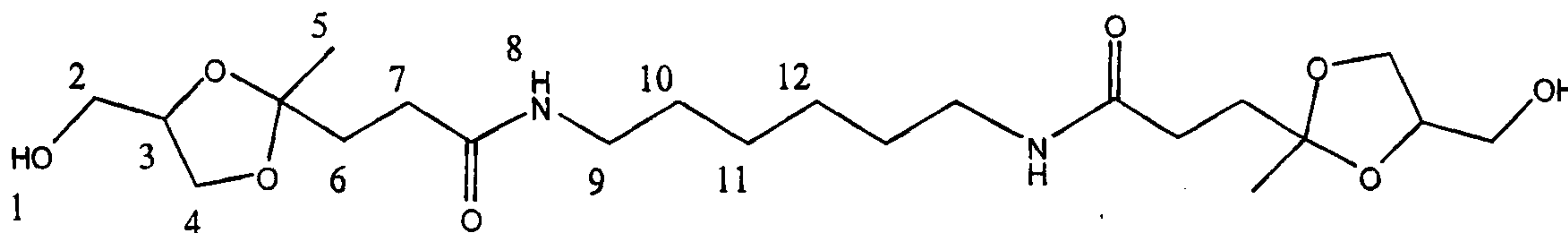
Proton assignments
