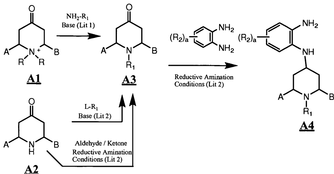
Scheme A
