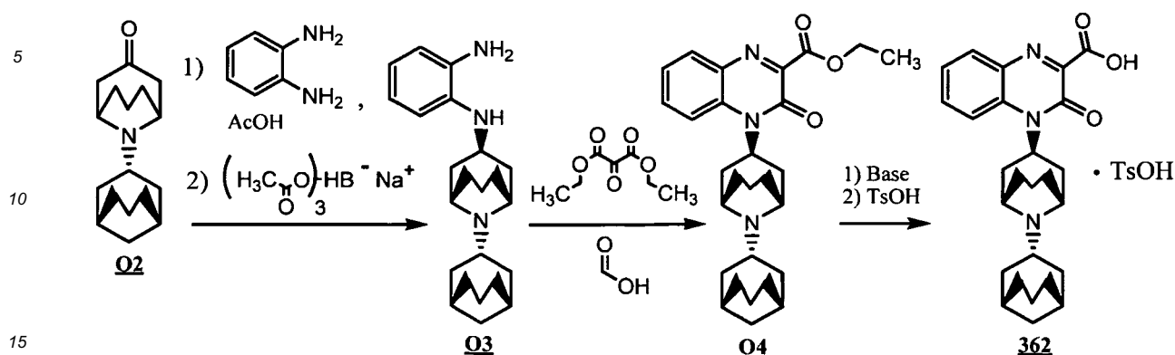
Scheme P
