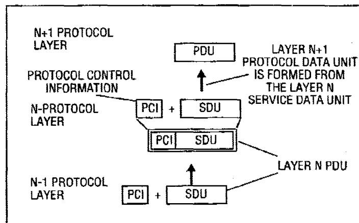
EGRESS OR RECEIVE PACKET RE-ASSEMBLY PROCESS
