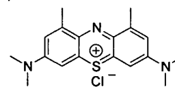
1,9-DIMETHYLMETHYLENE BLUE
