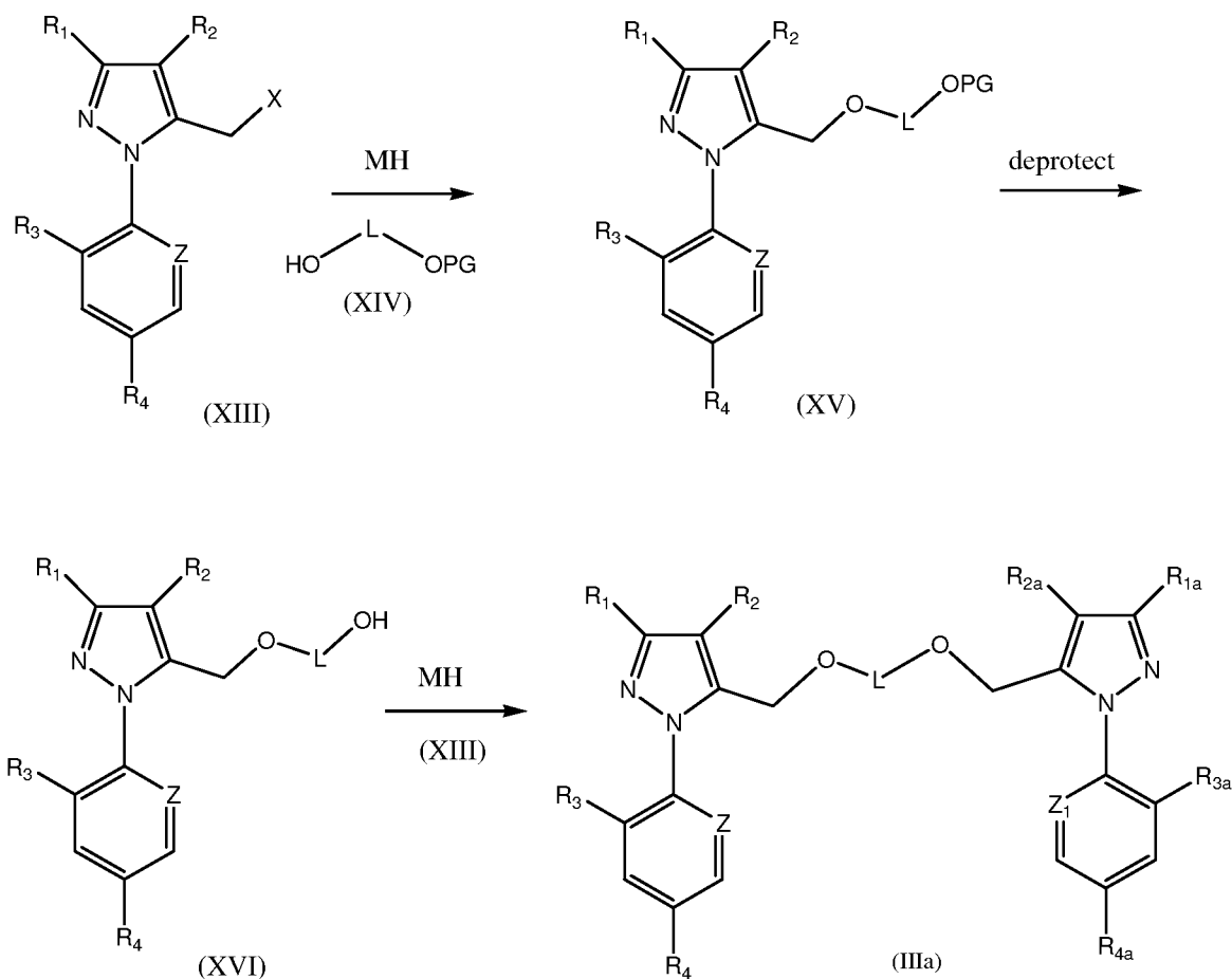
Scheme 3. Synthesis of compounds of formula (III) having linkers containing oxygen.
