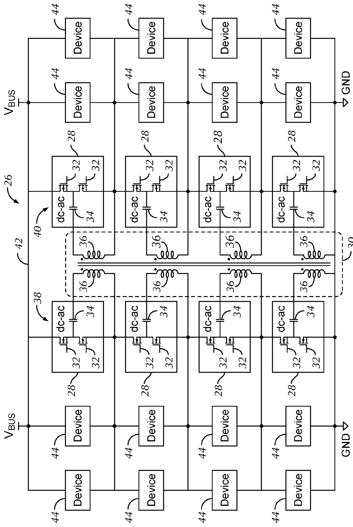
FIG. 2 Multiwinding Transformer
