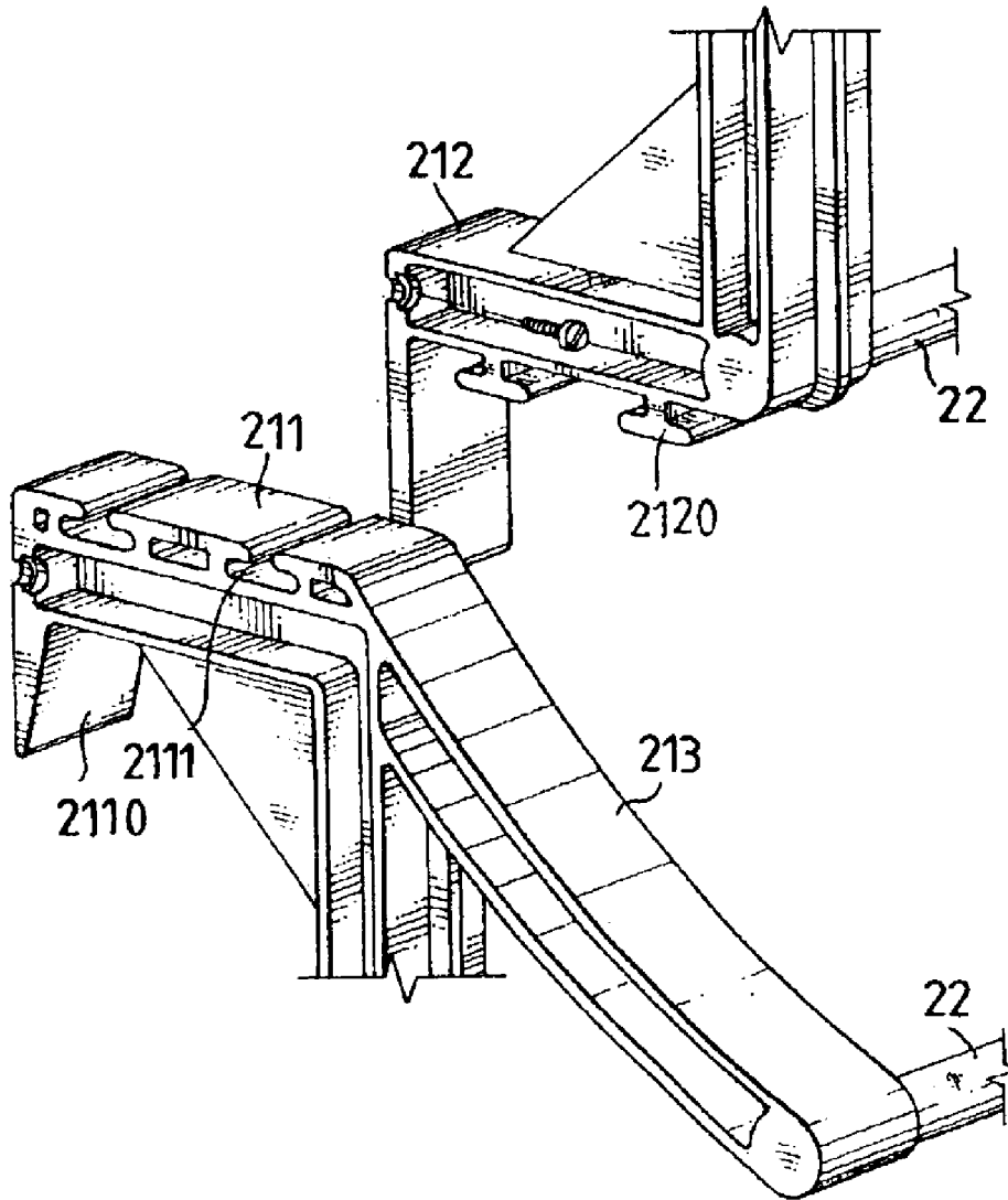
Fig. 2 PRIOR ART
