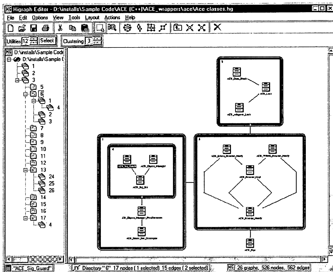
Fig. 13 – Node Expansion
