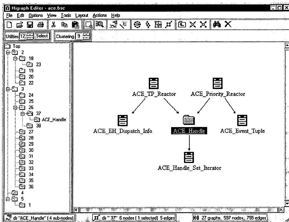
Fig. 3 – The Higraph Editor
