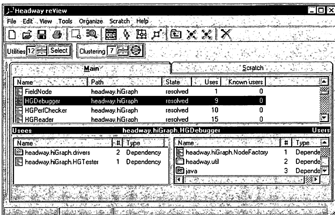
Fig. 10 – Dependency Viewer
