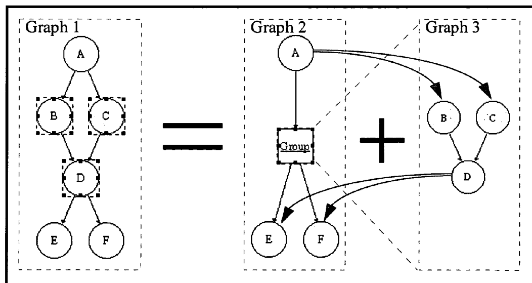
Fig. 2 - The Higraph Structure
