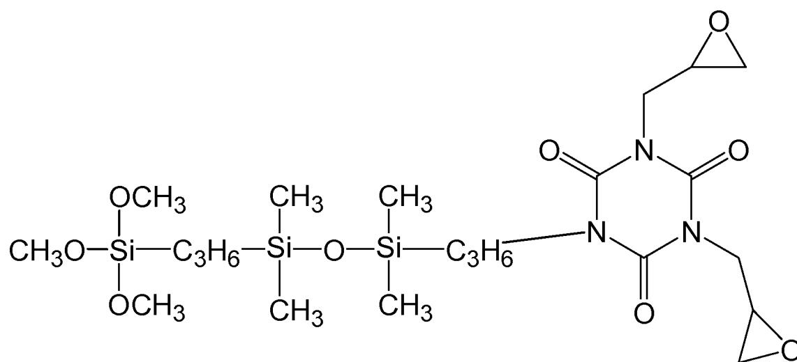
[Chemical Formula 16]
