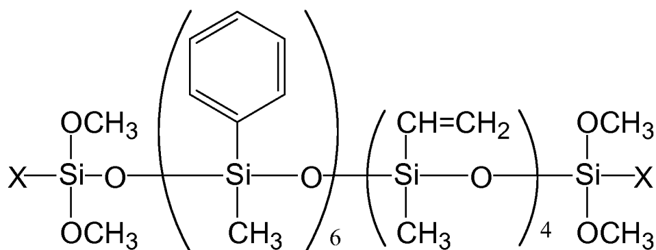
[Chemical Formula 21]
