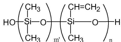
[Chemical Formula 7]
