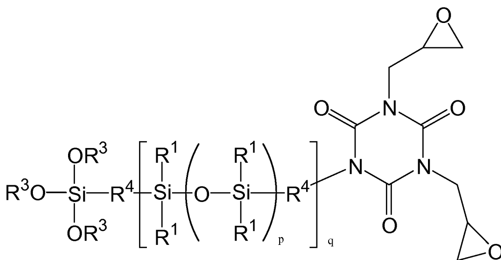
[Chemical Formula 6]
