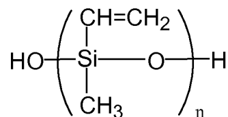
[Chemical Formula 8]
