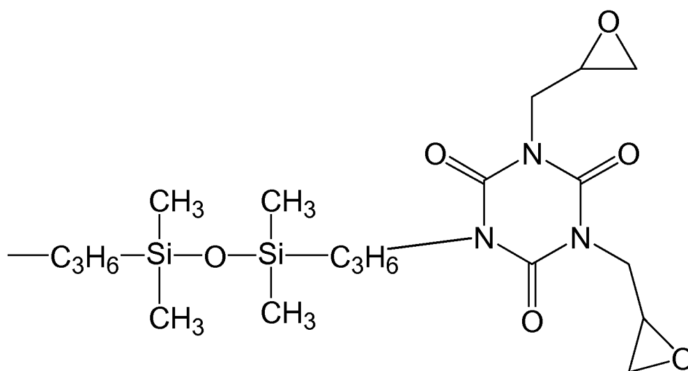
[Chemical Formula 14]
