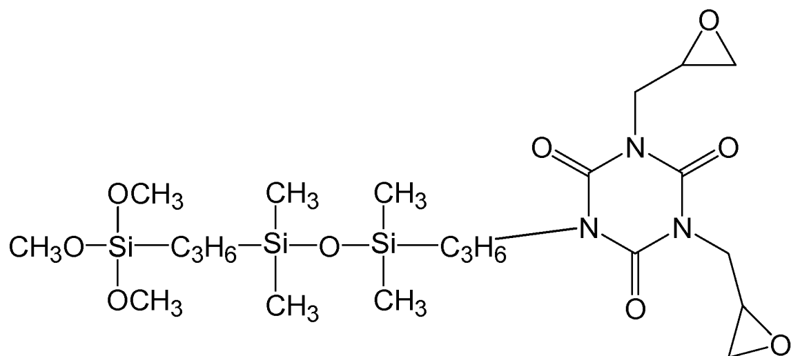
[Chemical Formula 20]
