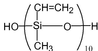
[Chemical Formula 15]
