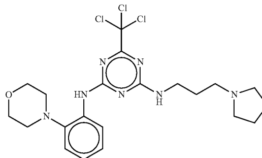
N²-(2-morpholinophenyl)-N⁴-(3-(pyrrolidin-1-yl)propyl)-6-(trichloromethyl)-1,3,5-triazine-2,4-diamine
