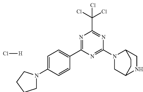
2-(4-(4-(pyrrolidin-1-yl)phenyl)-6-(trichloromethyl)-1,3,5-triazin-2-yl)-2,5-diazabicyclo[2.2.2]octane hydrochloride
