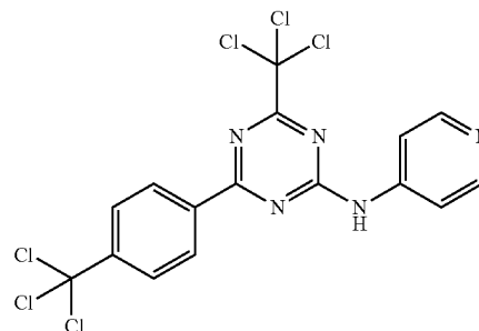
N-(pyridin-4-yl)-4-(trichloromethyl)-6-(4-(trichloromethyl)phenyl)-1,3,5-triazin-2-amine
