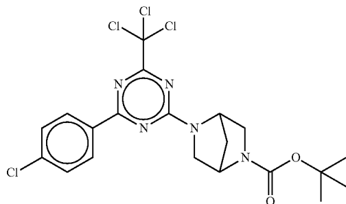
tert-butyl 5-(4-(4-chlorophenyl)-6-(trichloromethyl)-1,3,5-triazin-2-yl)-2,5-diazabicyclo[2.2.1]heptane-2-carboxylate
