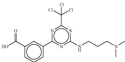
3-(4-((3-(dimethylamino)propyl)amino)-6-(trichloromethyl)-1,3,5-triazin-2-yl)benzoic acid
