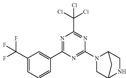
2-(4-(trichloromethyl)-6-(3-(trifluoromethyl)phenyl)-1,3,5-triazin-2-yl)-2,5-diazabicyclo[2.2.1]heptane
