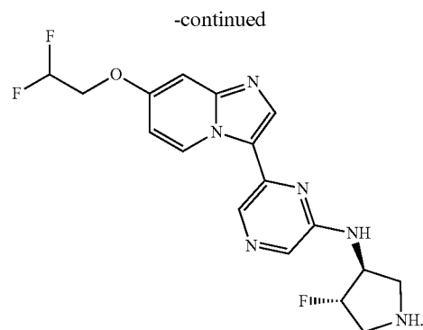
Formula (Ib)
