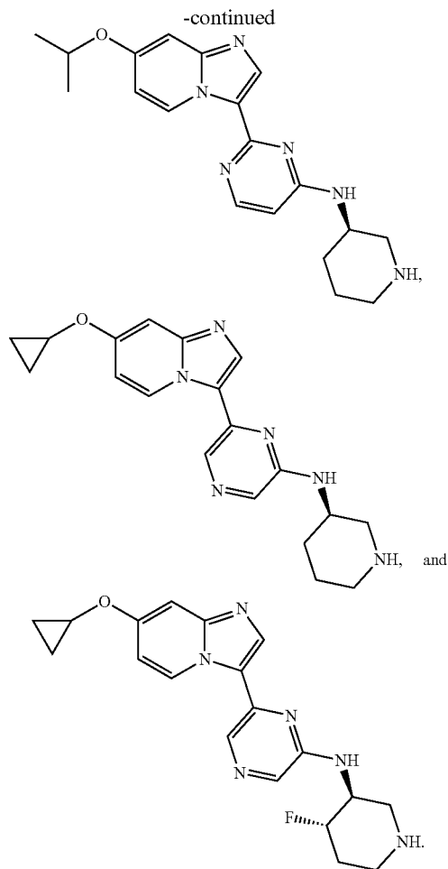
Formula (Id)
