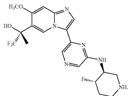
Formula (IIa)
