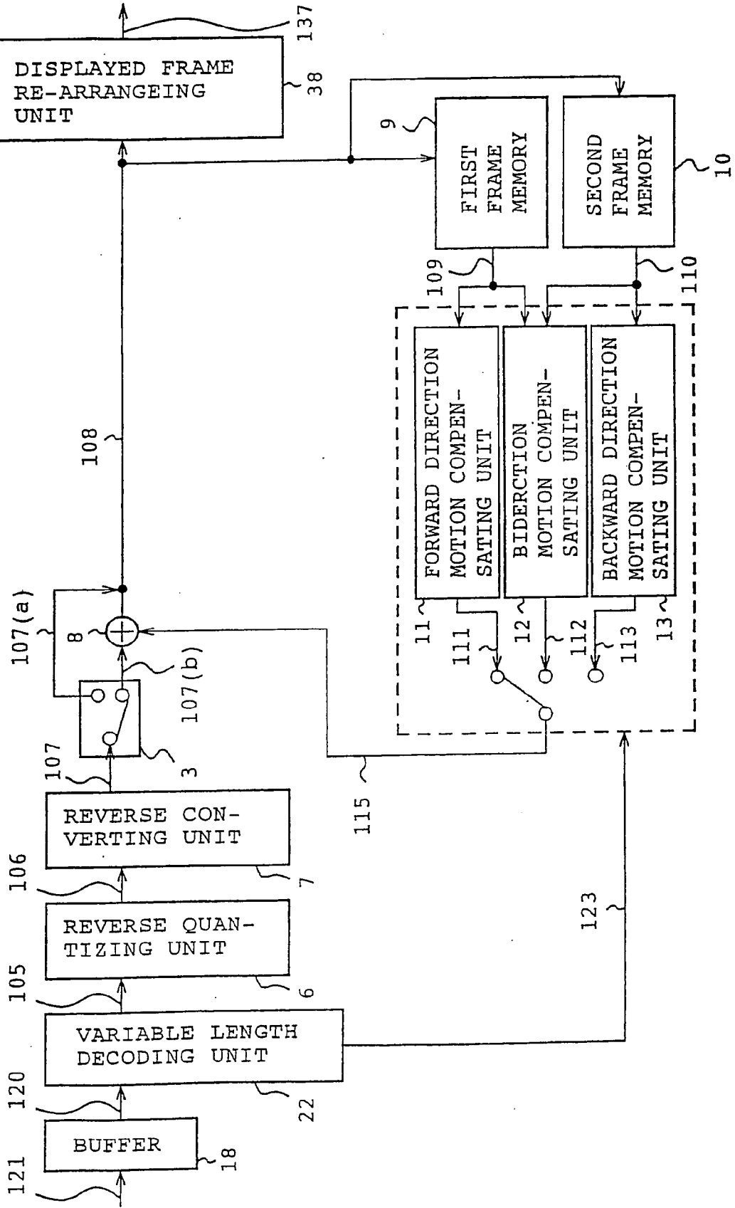
FIG. 19 (PRIOR ART)
