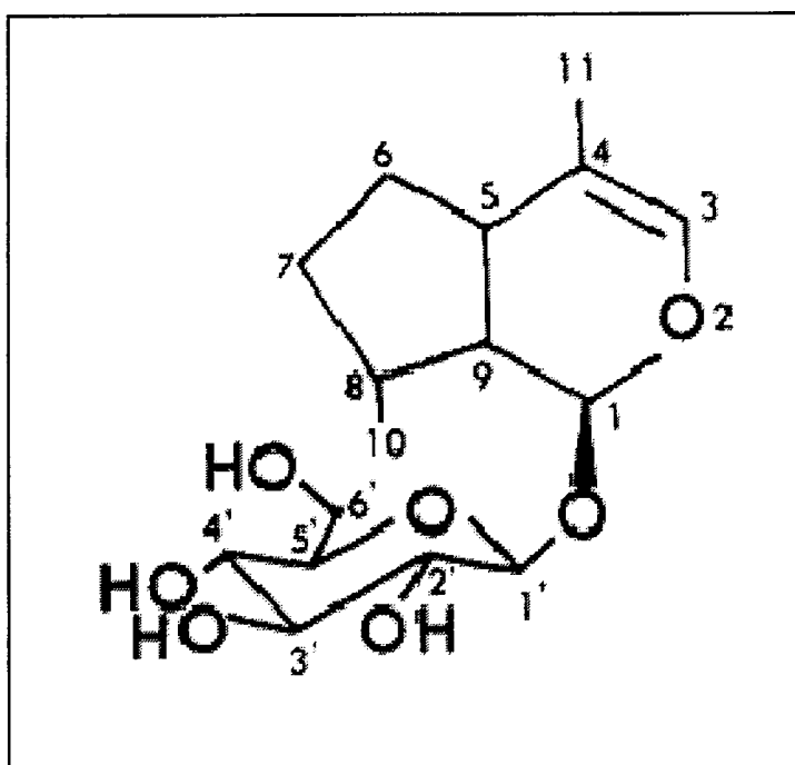
Iridoid
