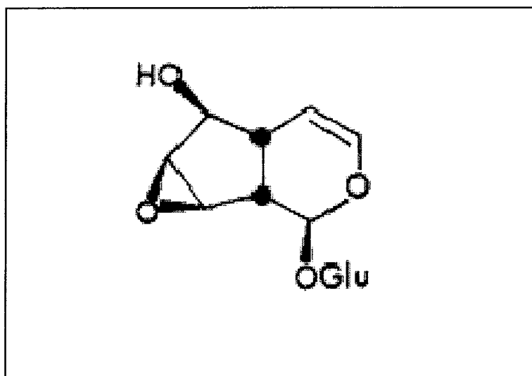
Glycosidic Iridoid
