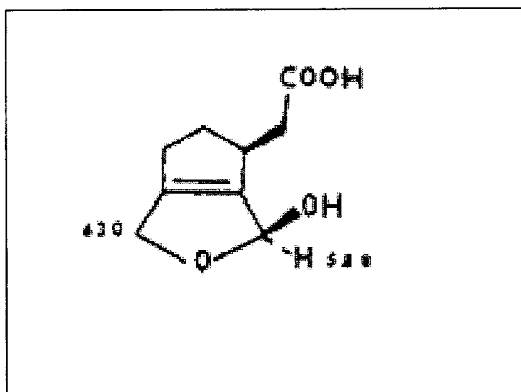
Non-Glycosidic Iridoid
