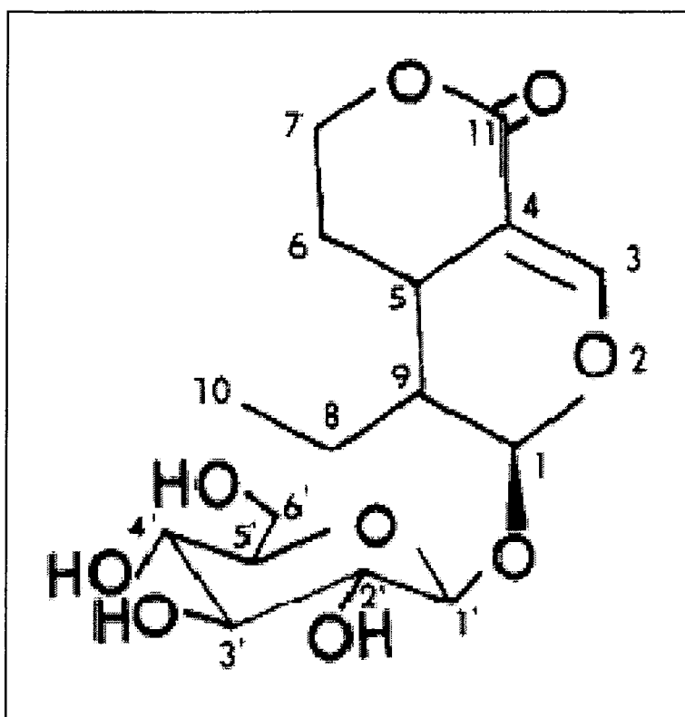
Secoiridoid
