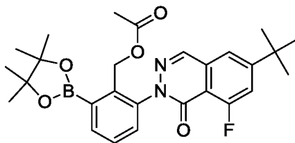
2-(6-( tert -butyl)-8-fluoro-1-oxophthalazin-2(1H)-yl)-6-(4,4,5,5-tetramethyl-1,3,2-dioxaborolan-2-yl)benzyl acetate
