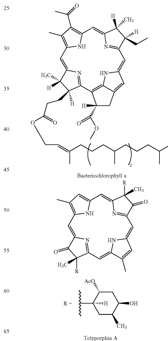
Scheme II
