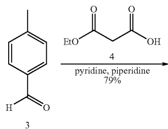
Scheme 3
