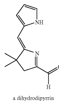
Chart 4
