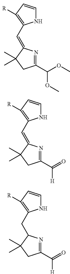
Chart 6
