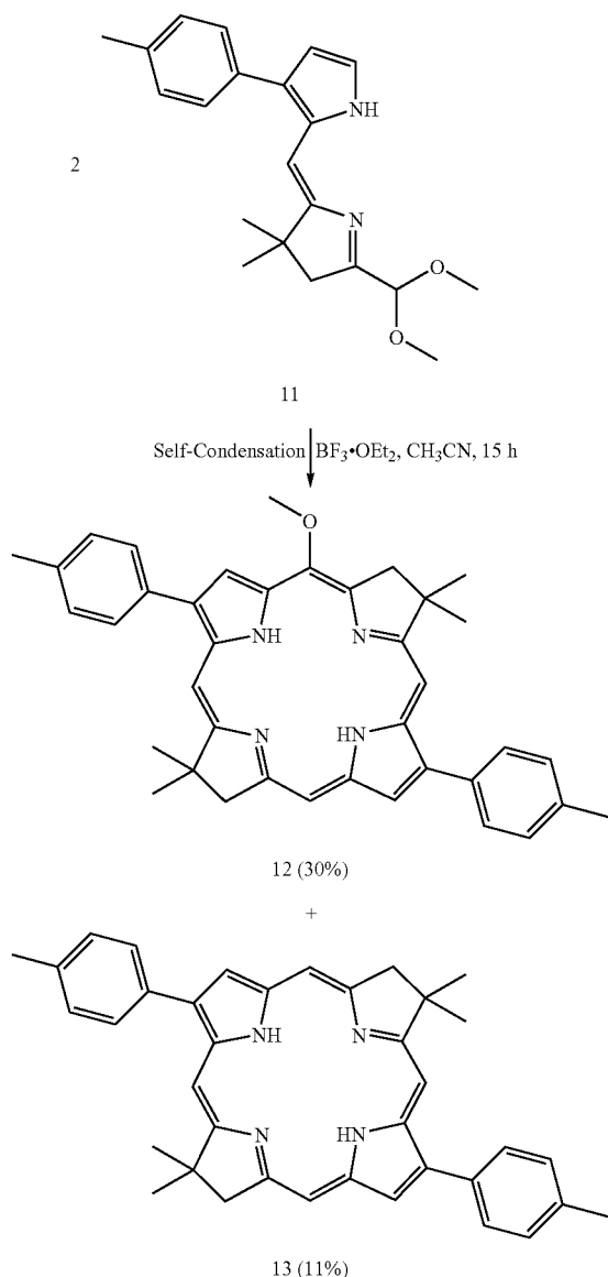
Scheme 4
