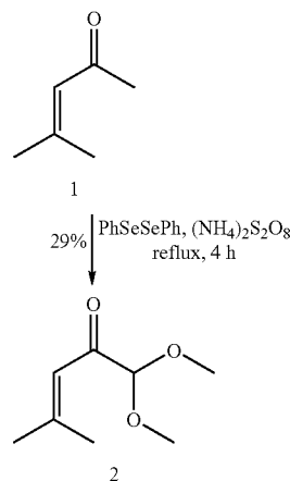
Scheme 2
