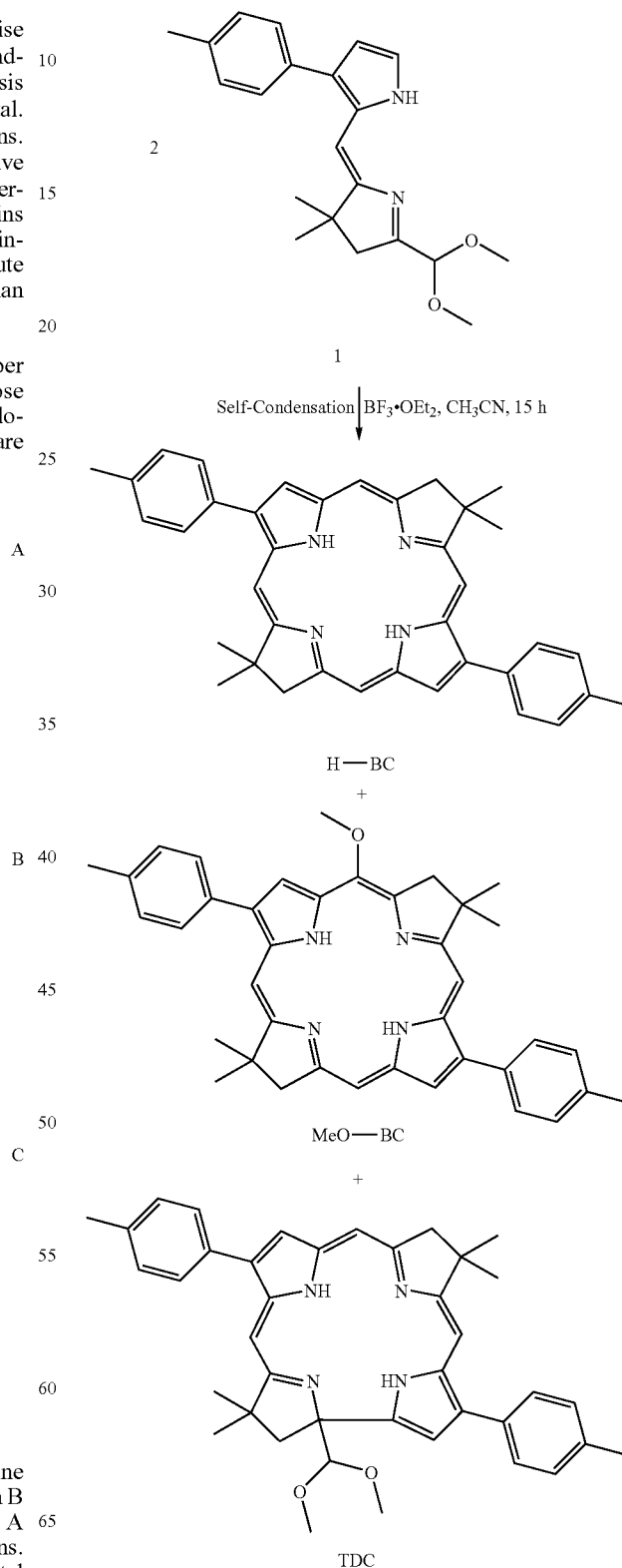
Scheme 6
