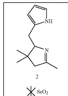
Scheme 8
