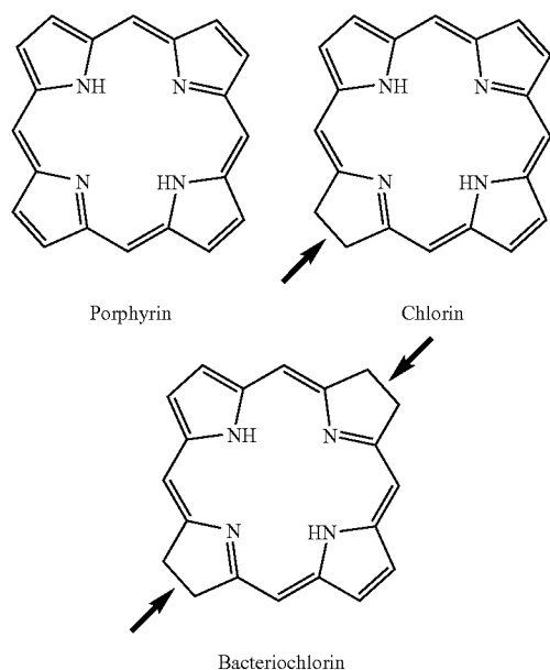
Scheme 1
