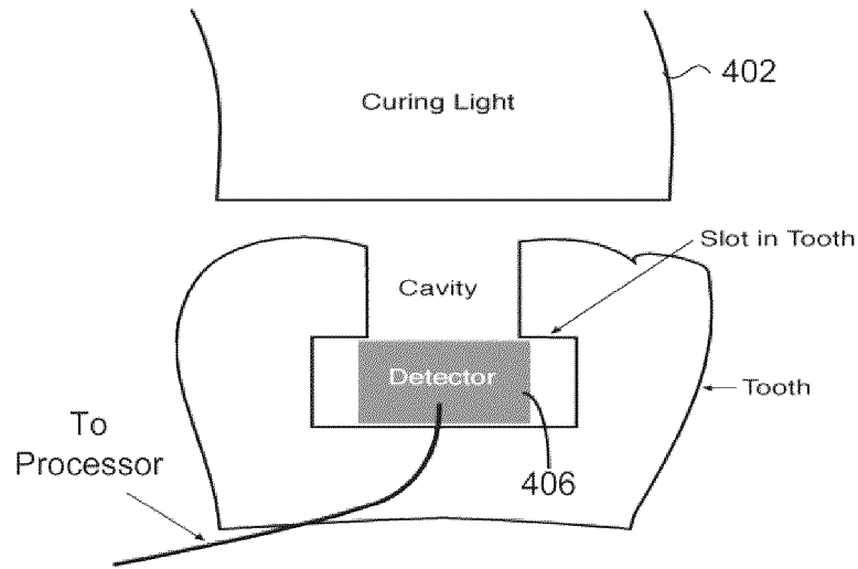
Cross Section
