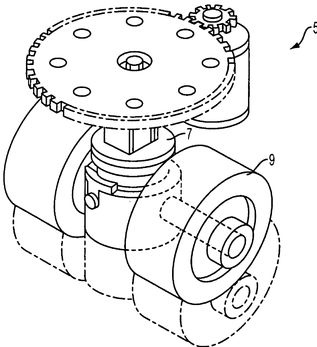
FIG. 1 PRIOR ART
