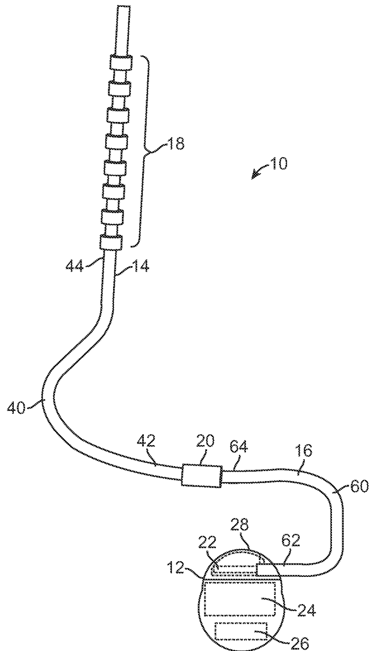
FIG. 1 (PRIOR ART)
