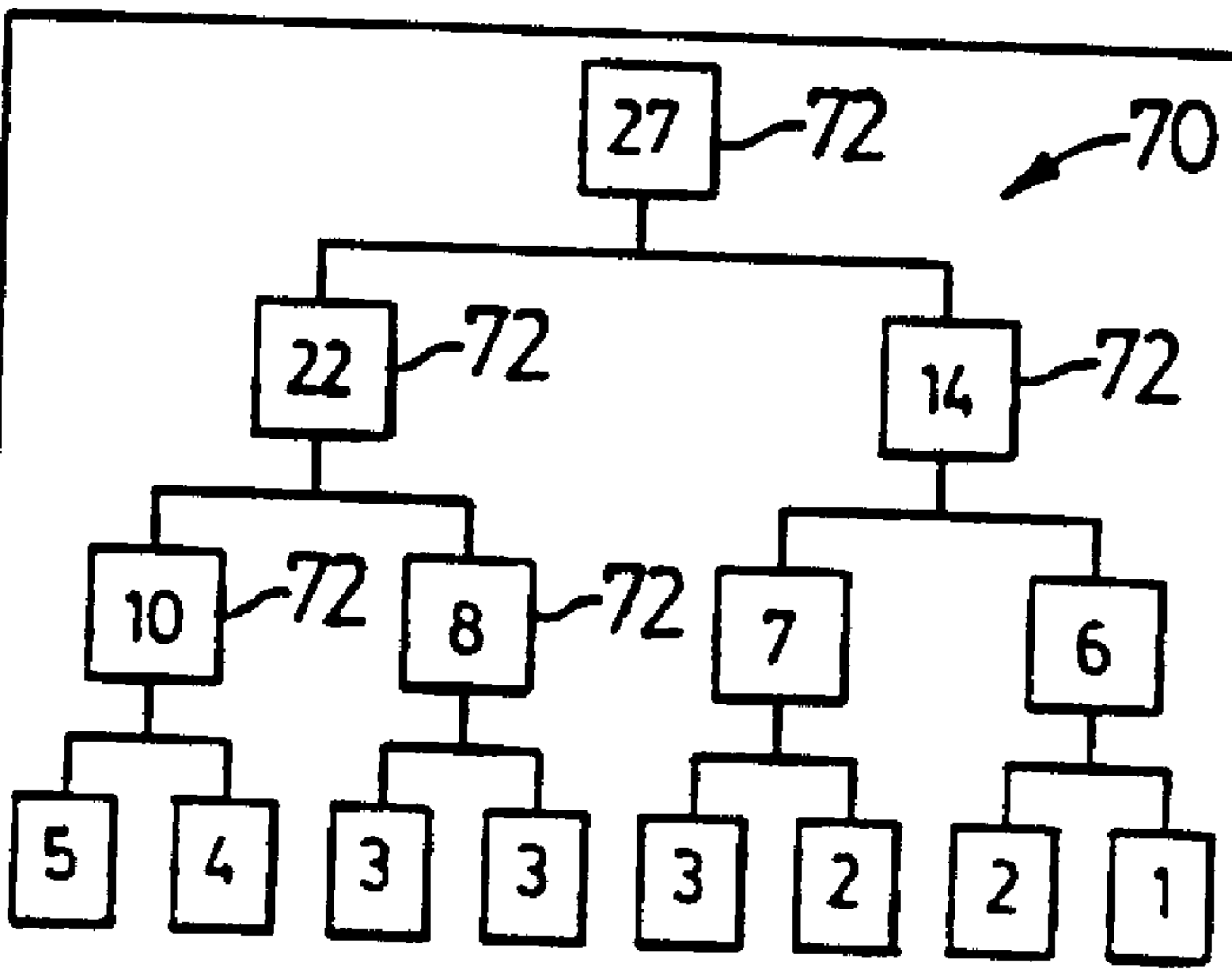
BALANCED SPANNING TREE FOR EXAMPLE 1
