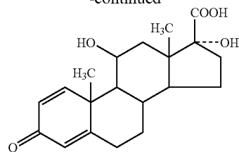
\Delta^1 -cortienic acid ( \Delta^1 -CA)
