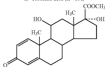
\Delta^1 -cortienic acid methyl ester ( \Delta^1 -MeCA)
