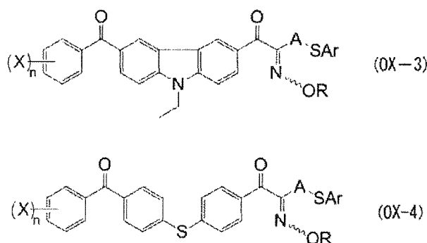
[Chem. 89]
