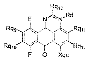
Formula (AQ-3)
