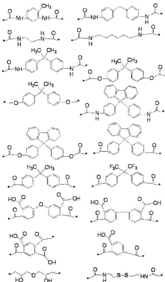
[Chem. 63]
