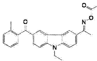
(I-2) IRUGACURE OXE02 (Manufactured by BASF)
