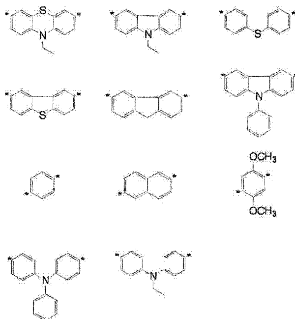
[Chem. 87]
