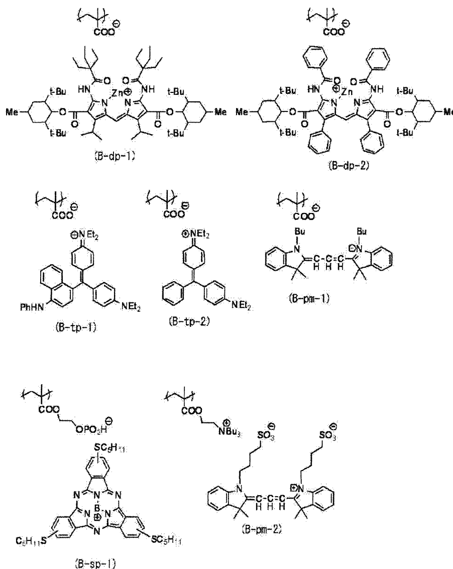
[Chem. 61]
