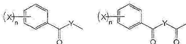
[Chem. 84]
