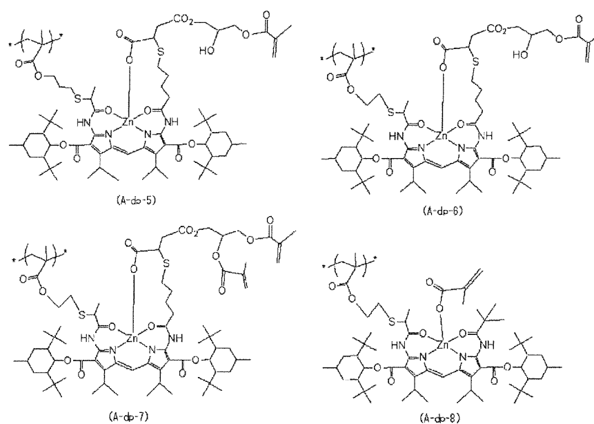
[Chem. 46]
