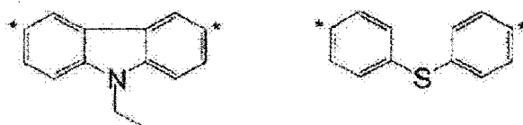
[Chem. 88]
