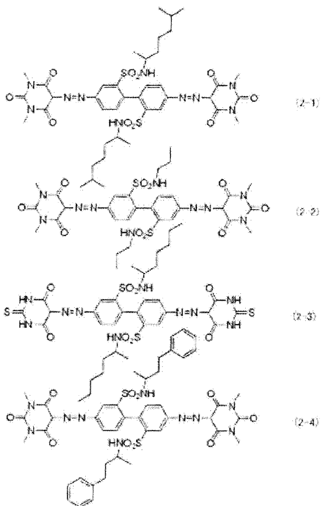
[Chem. 17]
