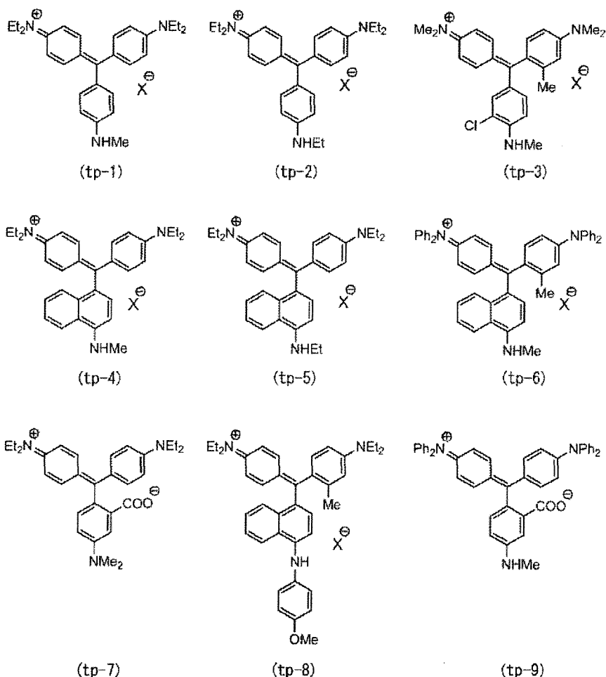
[Chem. 22]
