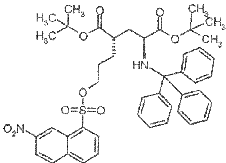
Di-tert-butyl (4S)-4-(3-[[[7-nitro-1-naphthyl)sulfonyl]oxy]propyl)-N-trityl-L-glutamat
