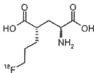
Formula IVa-F18
