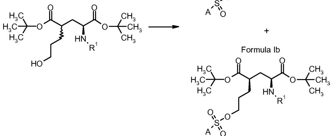
Formula IIa/b
