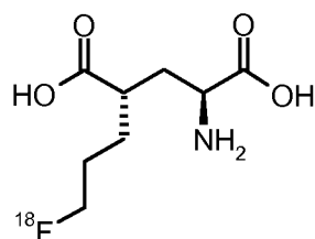
Formula IVa-F18
