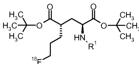
Formula IIla-F18
