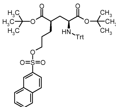
di- tert -butyl (4 R )-4-{3-[(2-naphthylsulfonyl)oxy]propyl}- N -trityl-L-glutamate ( Ik )
