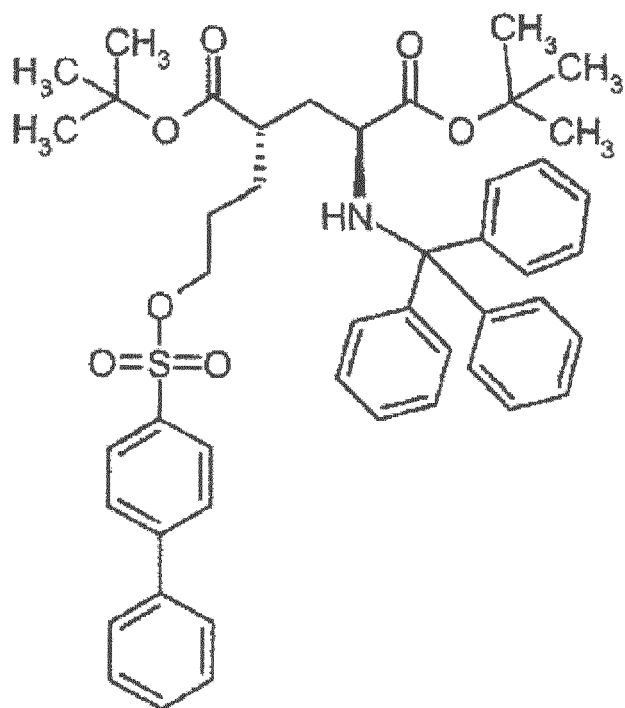
Di-tert-butyl (4S)-4-{3-[(2-naphthylsulfonyl)oxy]propyl}-N-trityl-L-glutamat
