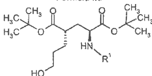
Formula IIa
