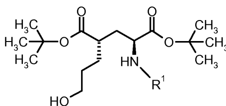
Formula IIa
