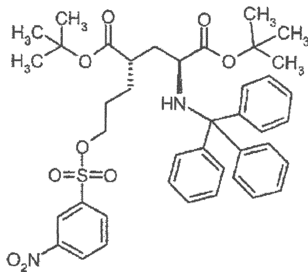
di-tert-butyl (4S)-4-(3-((biphényl-4-yl)sulfonyl)oxy)propyl)-N-trityl-L-glutamate
