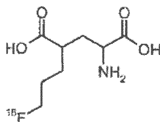
Formula IV-F18
