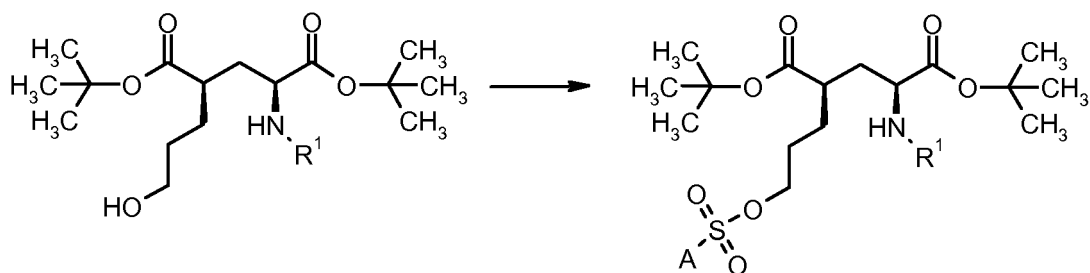
Formula Ib
