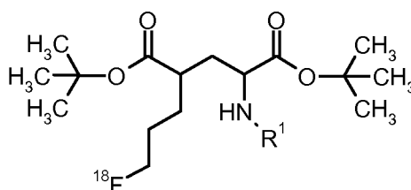
Formula III-F18
