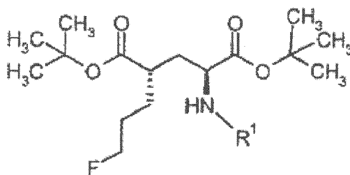
Formula IIIa-F
