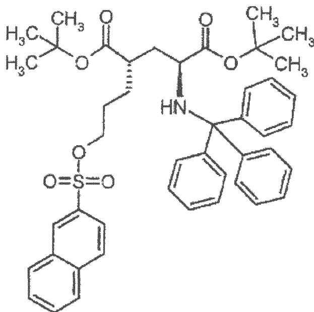
di-tert-butyl (4S)-4-{3-[(1-naphthylsulfonyl)oxy]propyl}-N-trityl-L-glutamate
