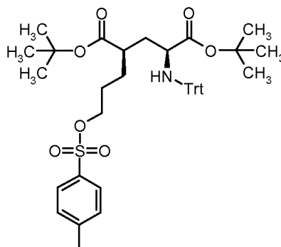
di- tert -butyl (4 R )-4-{3-[(4-methylphenyl)sulfonyl]oxypropyl}- N -trityl-L-glutamate ( In )
