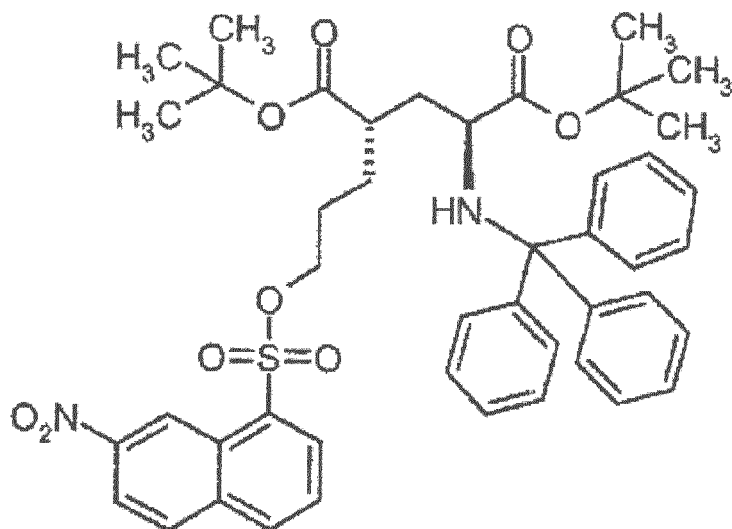
di-tert-butyl (4S)-4-(3-[[[7-nitro-1-naphthyl)sulfonyl]oxy]propyl)-N-trityl-L-glutamate
