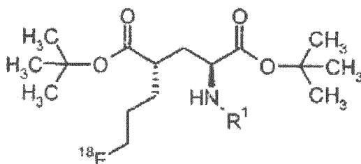
Formula IIIa-F18
