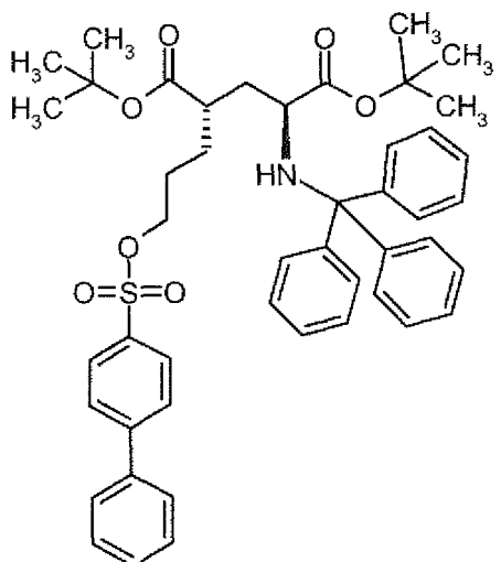
Di-tert-butyl (4S)-4-{3-[(2-naphthyl)sulfonyl]oxy}propyl)-N-trityl-L-glutamate
