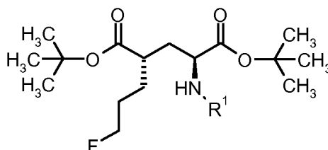
Formula IIIa-F
