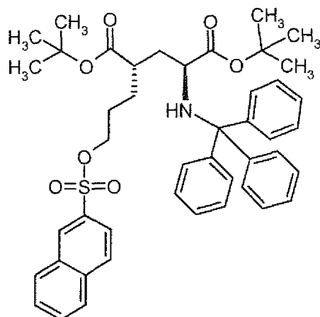
Di-tert-butyl (4S)-4-{3-[(1-naphthylsulfonyl)oxy]propyl}-N-trityl-L-glutamate
