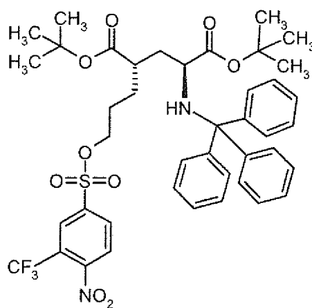
di-tert-butyl (4S)-4-(3-{{[4-methylphenyl]sulfonyl}oxy}propyl)-N-trityl-L-glutamate.
