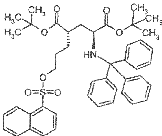
Di-tert-butyl (4S)-4-{3-[(chinolin-8-ylsulfonyl)oxy]propyl}-N-trityl-L-glutamat
