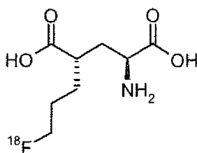
Formula IVa-F18
