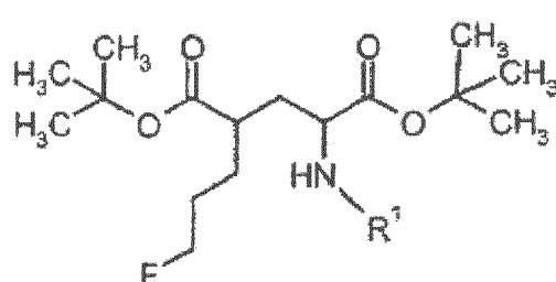
Formula III-F
