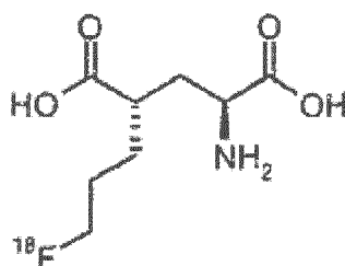
Formula IVa-F18
