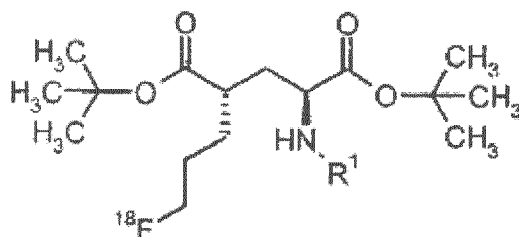
Formula IIIa-F18
