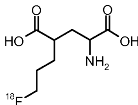
Formula IV-F18
