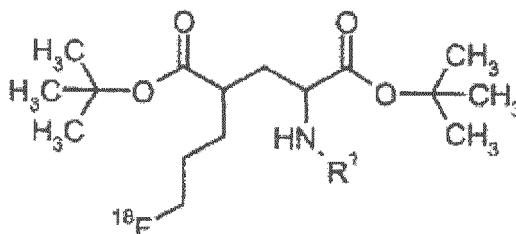
Formula III-F18
