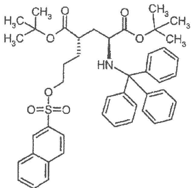
Di-tert-butyl (4S)-4-{3-[(1-naphthylsulfonyl)oxy]propyl}-N-trityl-L-glutamat
