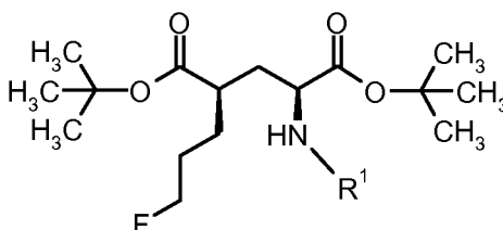
Formula IIIb-F
