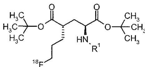
Formula IIIa-F18
