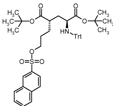
di- tert -butyl (4 S )-4-{3-[(2-naphthylsulfonyl)oxy]propyl}- N -trityl-L-glutamate ( Id )
