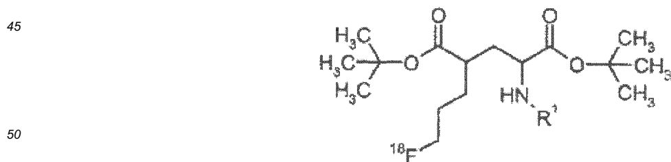
Formula III-F18
