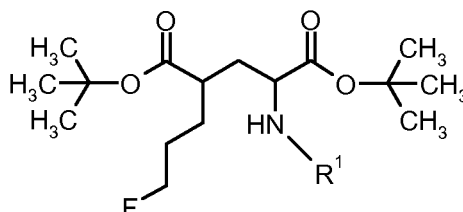
Formula III-F
