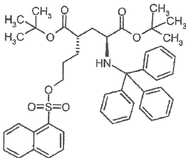
di-tert-butyl (4S)-4-{3-[(quinolin-8-ylsulfonyl)oxy]propyl}-N-trityl-L-glutamate
