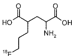
Formula IV-F18
