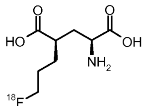
Formula IVb-F18
