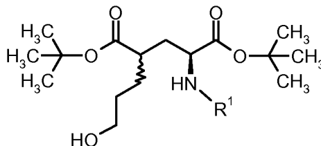
Formula IIa/b
