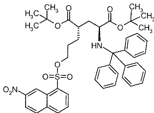
Di-tert-butyl (4S)-4-[3-({[4-nitro-3-(trifluoromethyl)phenyl]sulfonyl}oxy)propyl]-N-trityl-L-glutamate
