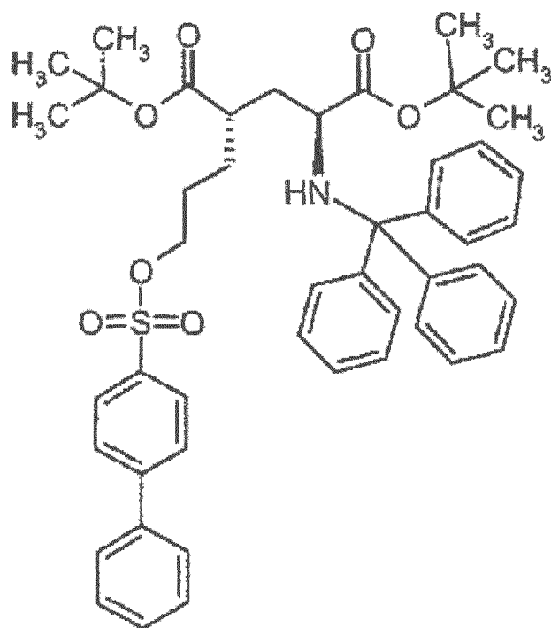
di-tert-butyl (4S)-4-{3-[(2-naphthylsulfonyl)oxy]propyl}-N-trityl-L-glutamate
