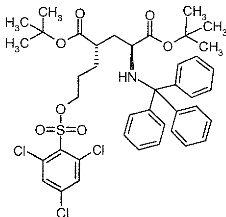
Tetra-tert-butyl (2S,4S,2'S,4'S)-2,2'-[biphenyl-4,4'-diylbis(sulfonyloxopropane-3,1-diyl)]bis[4-(tritylamino)pentanedioate]
