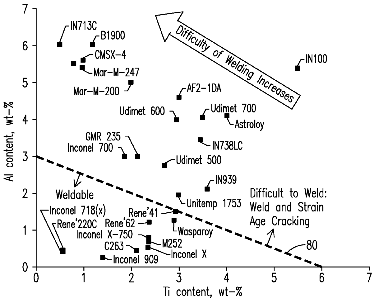
FIG. 9 PRIOR ART
