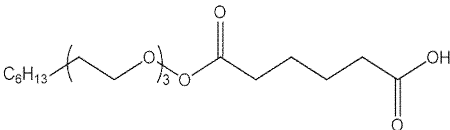
[Chemical Formula 1-3]
