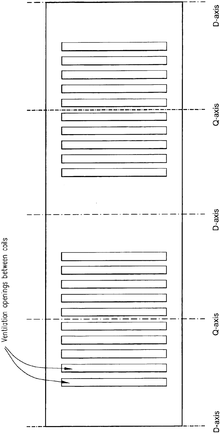
Fig.5 Single Piece Ventilated Shield
