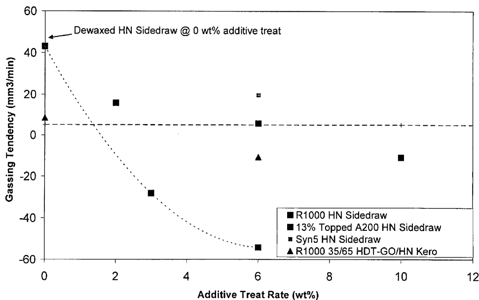
A200: Larger Gassing Tendency Response vs Alternatives
