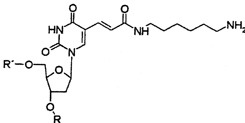
Formula I
