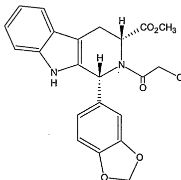
Compound V
