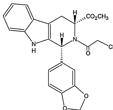
Compound V
