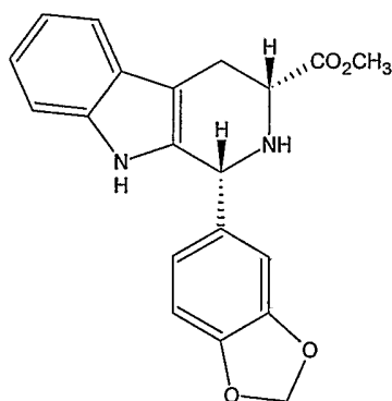
Compound III
