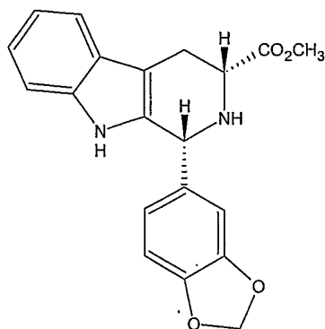
Compound III
