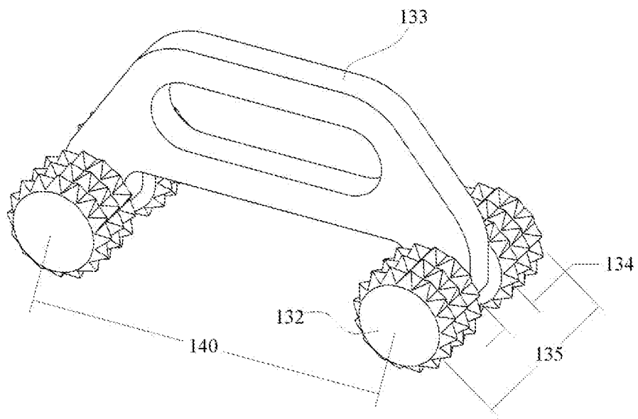
FIG. 11 (PRIOR ART)
