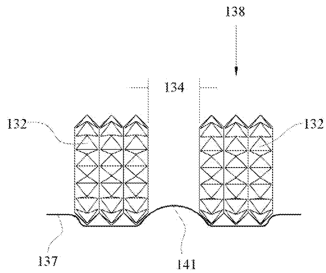
FIG. 13 (PRIOR ART)
