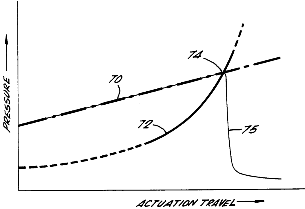
FIG. 6. PRESSURE DIAGRAM
