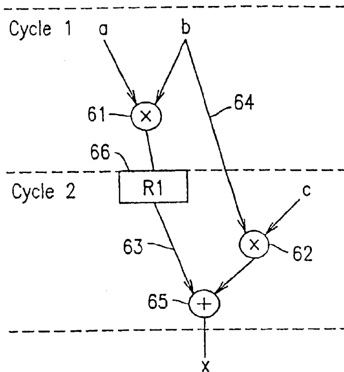
FIG. 6 CONVENTIONAL ART
