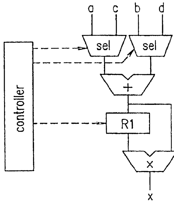
FIG. 10 CONVENTIONAL ART
