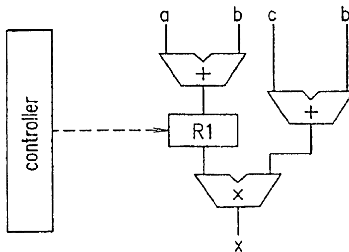
FIG. 11 RELATED ART
