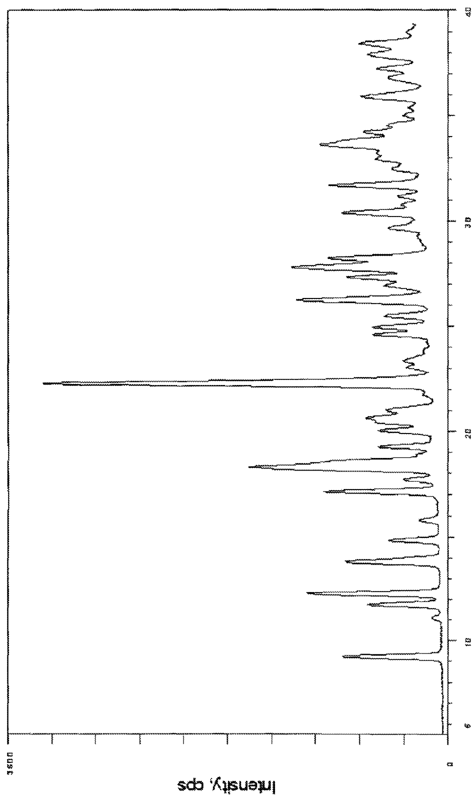
2 theta Figure 4
