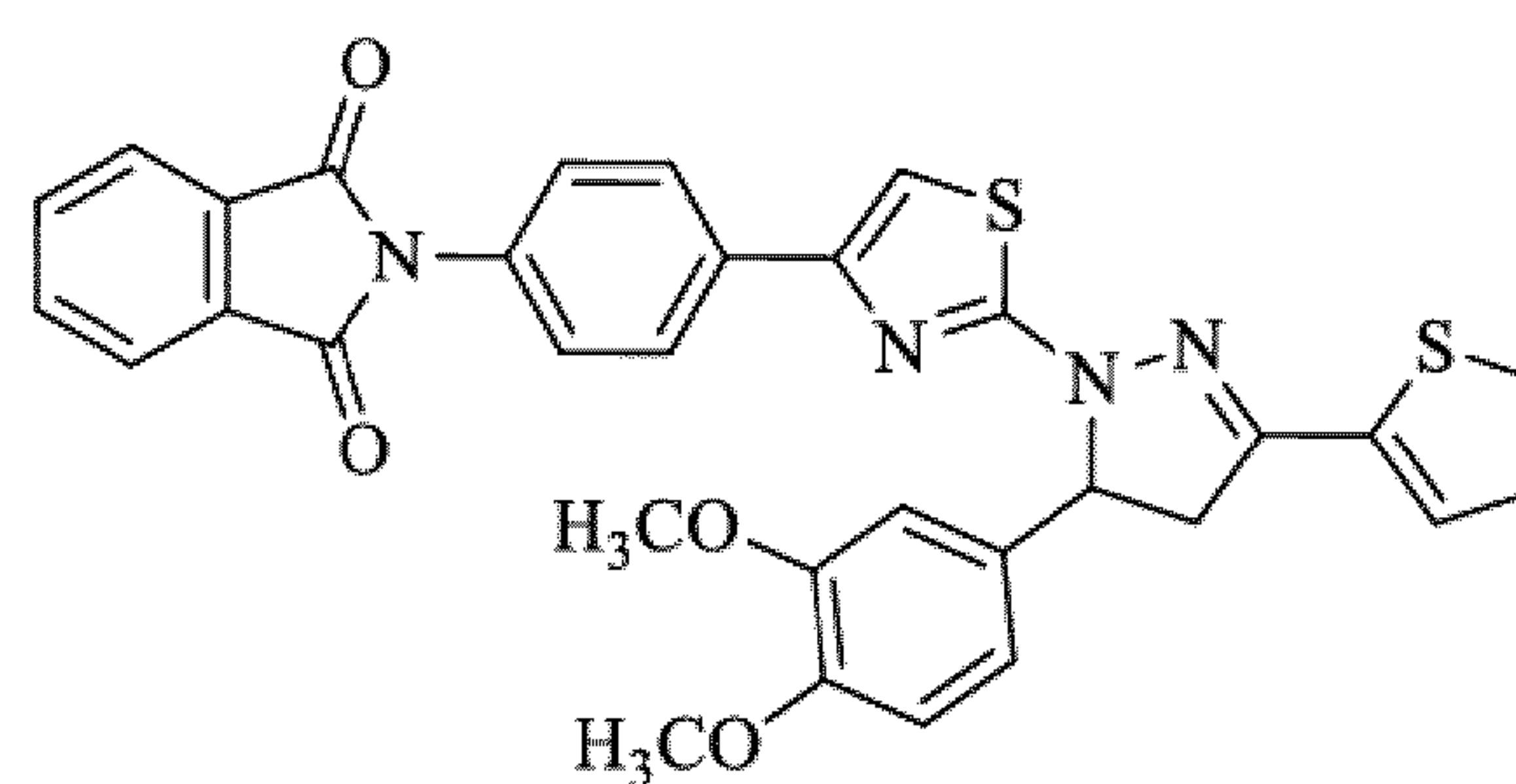
compound a
