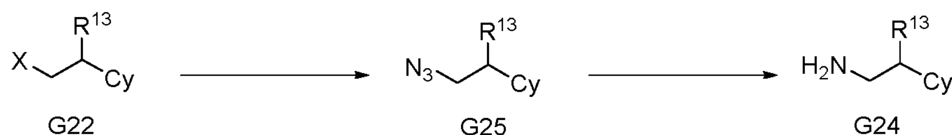
Scheme 10B
