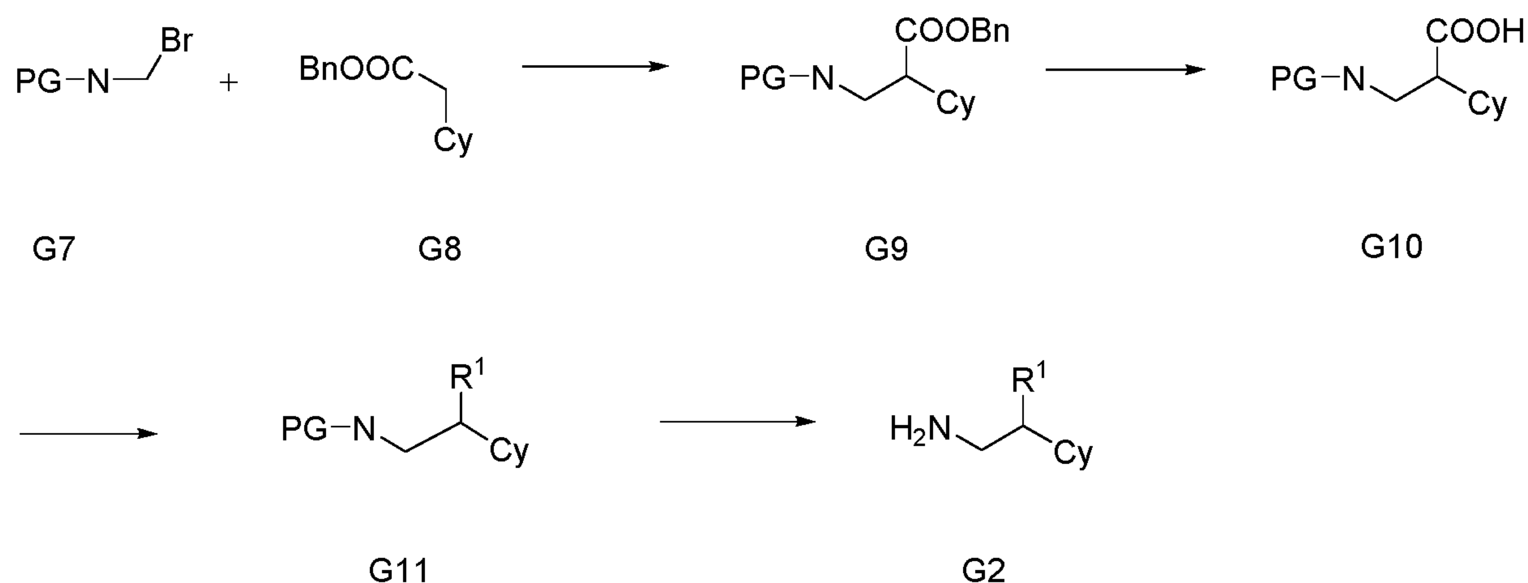
Scheme 5A
