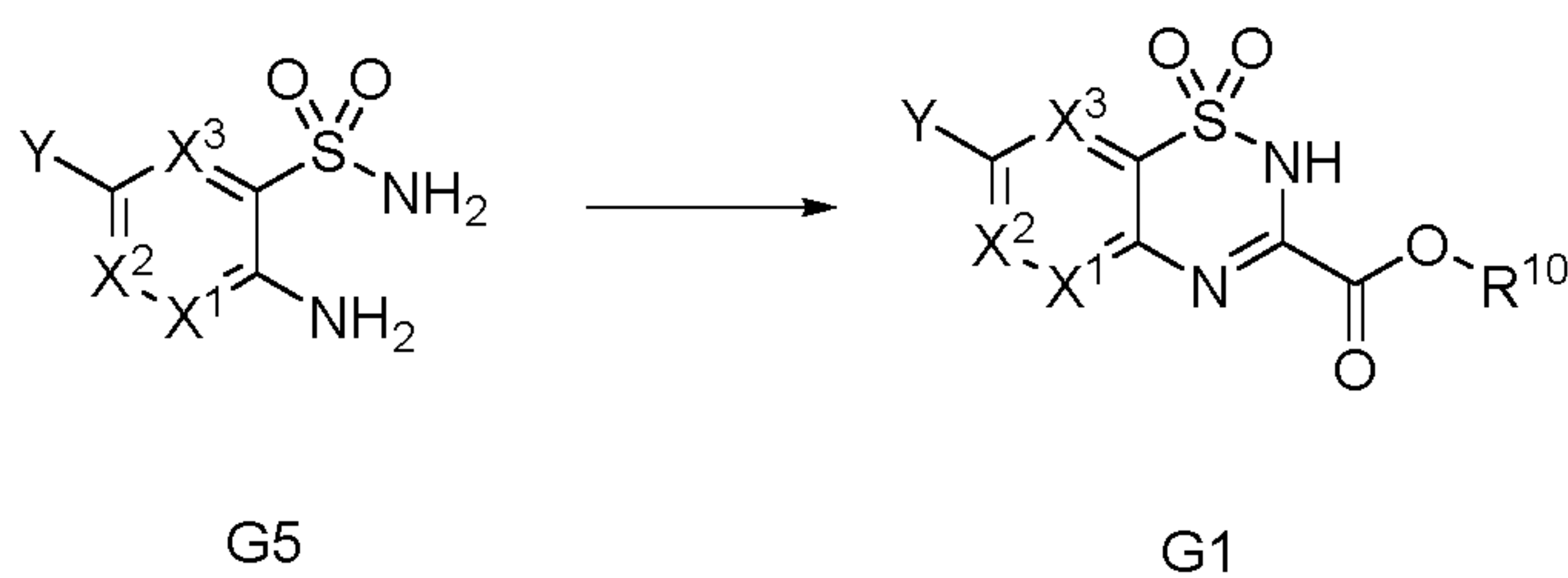
Scheme 4A
