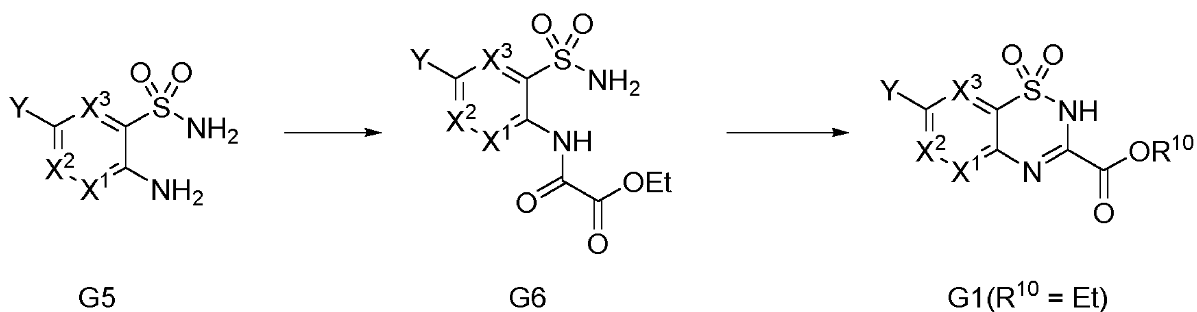
Scheme 3A
