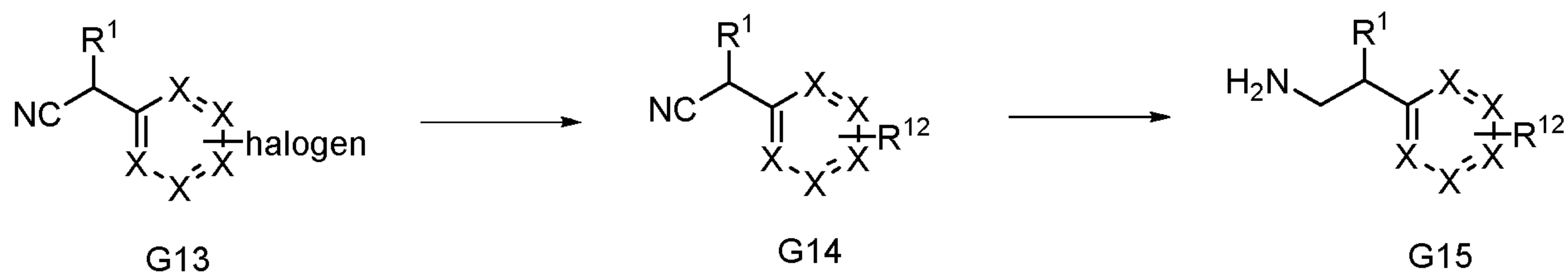
Scheme 7A
