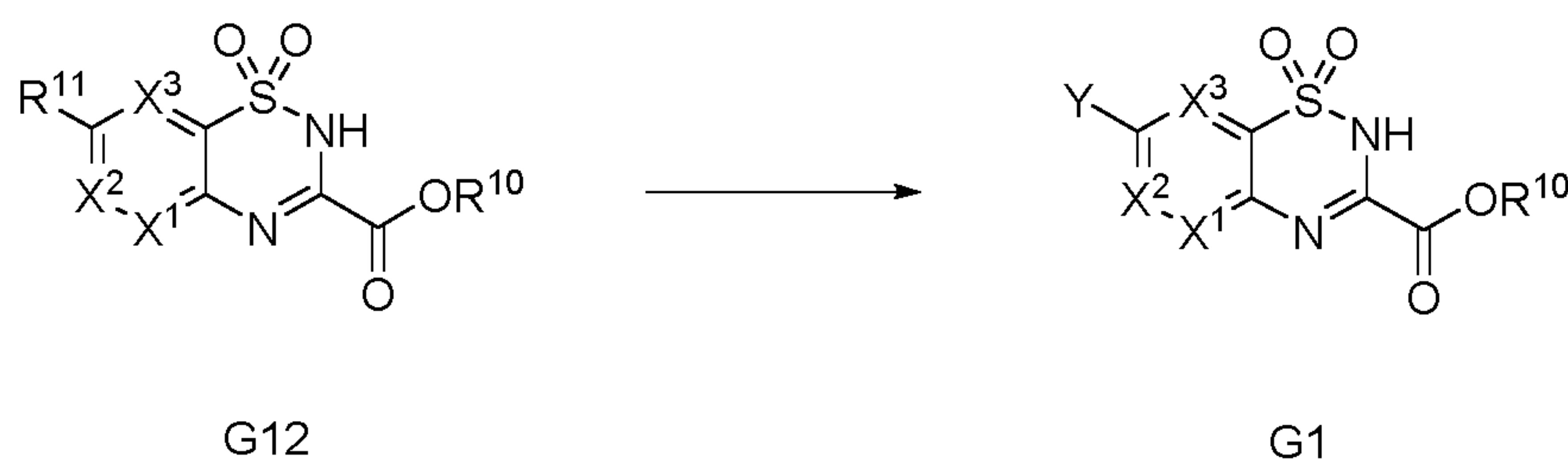
Scheme 6A
