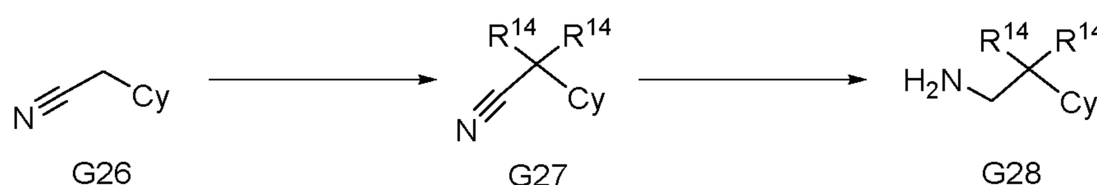
Scheme 11A
