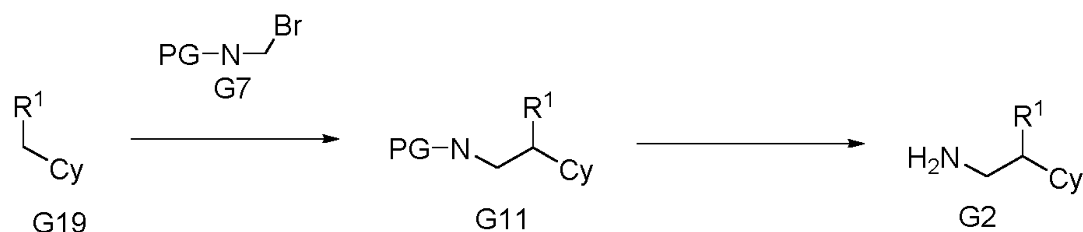
Scheme 8B
